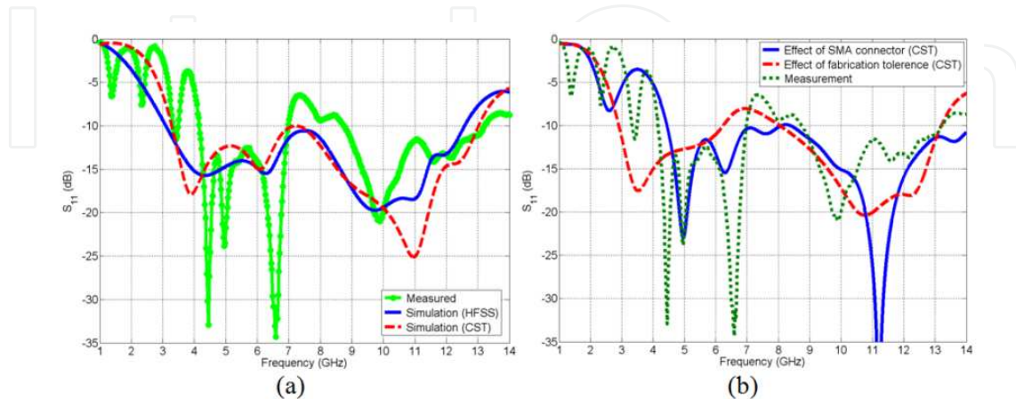
Figure 17. (a) Measured and simulated reflection coefficient curves of the maple-leaf antenna (b) effect of fabrication tolerance on the performance of maple-leaf antenna.
