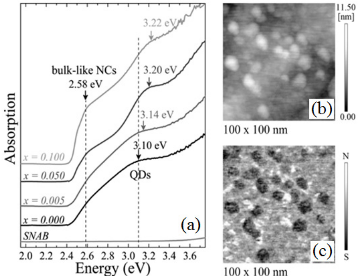
Figure 1. (a) Room temperature OA spectra of Cd_{1-x}Mn_xS NPs with different x -concentrations embedded in the SNAB glass matrix. The two groups of NPs (QDs and bulk-like NCs) are indicated by the vertical dashed lines. The OA spectrum of the SNAB glass matrix is also shown at the bottom for comparison. (b) Topographic MFM image showing high quantities of Cd_{0.900}Mn_{0.100}S NPs at the sample's surface, and (c) the corresponding phase MFM image (30 nm lift) where the contrast between the North (N) and South (S) magnetic poles identifies the orientation of the total magnetic moment of the DMS NPs.
