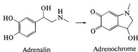
Figure 17. Structures of adrenalin and adrenochrome
