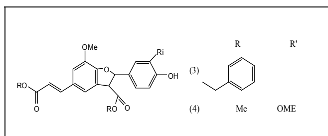
Figure 10. Structures of Xanthene (MF1, MF2) and neo-lignans (MF3, MF4)
