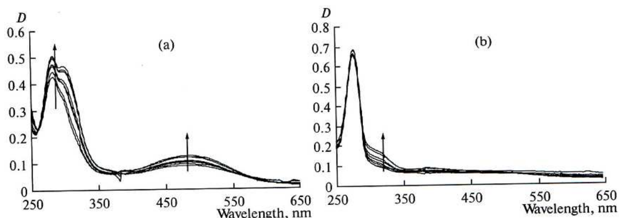
Figure 16. Variations in UV spectrum of 0.1 mM adrenaline solution in the process of its oxidation at 37°C (a) in water and 0.9% NaCl solution and (b) in phosphate buffer with pH 7.2.
