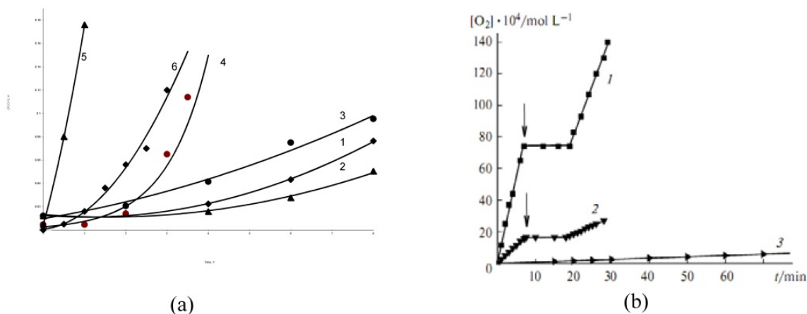
Figure 12. (a). Effect of surfactant on the LOOH formation during autoxidation of TGOO at 100°C and TGSO at 80°C: 1, 4- without additives; 3, 5 - 0.1M CTAB; 2, 4- 0.1 M SDS; 6 - 0.04 M 1-OD [48]; (b) Effect of surfactant on the oxygen absorption during 1M limonene oxidation at 60°C; 1 – 1mM CTAC; 2 – 0,8 mM CTAB; 3 – 1mM SDS; 3- without additives; [LOOH]=22mM; Arrows show the moments of introducing \alpha -tocopherol: 1-0,8 mM; 2 – 0,2 mM [51].
