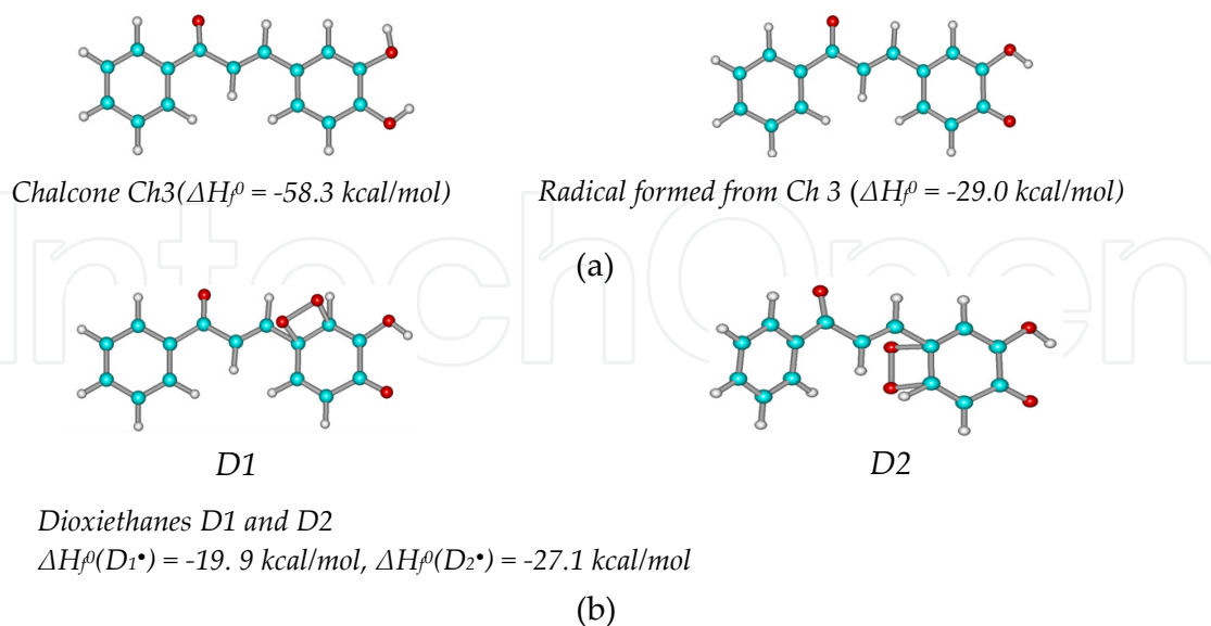
Figure 7. a) Optimized structures of Chalcone Ch3 (7a) and its aryl radical (7b); b) Optimized structures of Dioxietanes D1 and D2 formed from Ch3 radical and oxygen.
