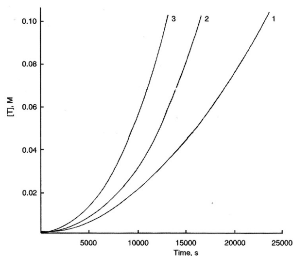
Figure 2. Influence of dimer formation equilibrium constant ( K_2 ) on the kinetics of MeLi autoxidation at 60^\circ\text{C} , when e_2 k_{32} has a great value ( e_2 k_{32} = 2 \cdot 10^{-6} ), [\text{T}_0] = 10^{-4} \text{M} , d = 2 \cdot 10^{-7} and k_p / (k_t)^{1/2} = 6 \cdot 10^{-2}
