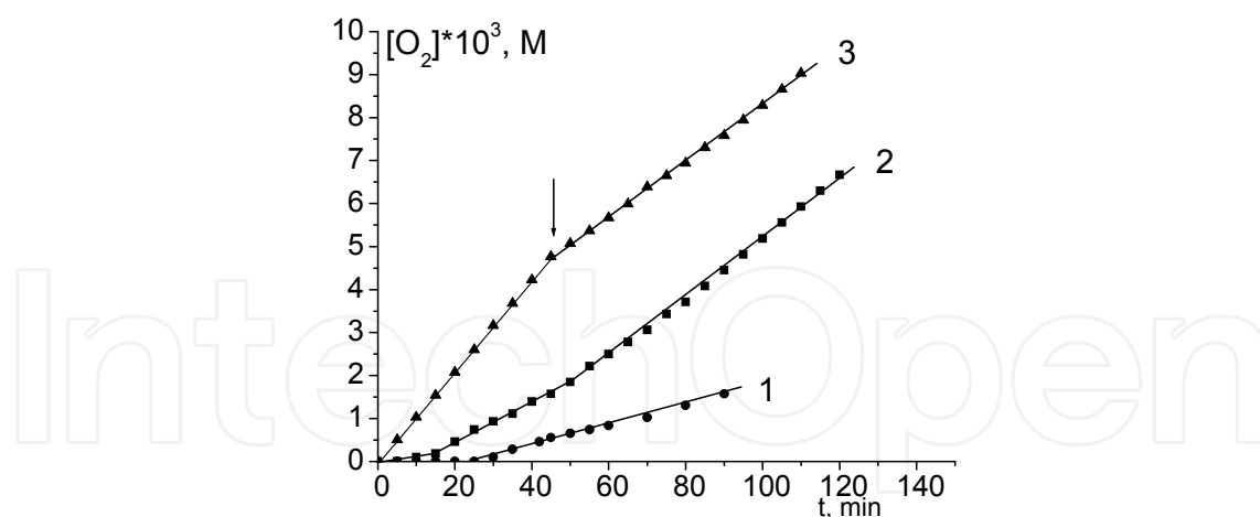
Figure 14. Kinetic curves for O_2 absorption during AAPH-initiated (55 mM) oxidation of PL (45 mg/ml) in water at 37^\circ C in the presence of (1) 0.33 and (2) 0.05 mM \alpha -tocopherol incorporated upon preparation of liposomes and (3) 0.05 mM \alpha -tocopherol introduced directly into solution
