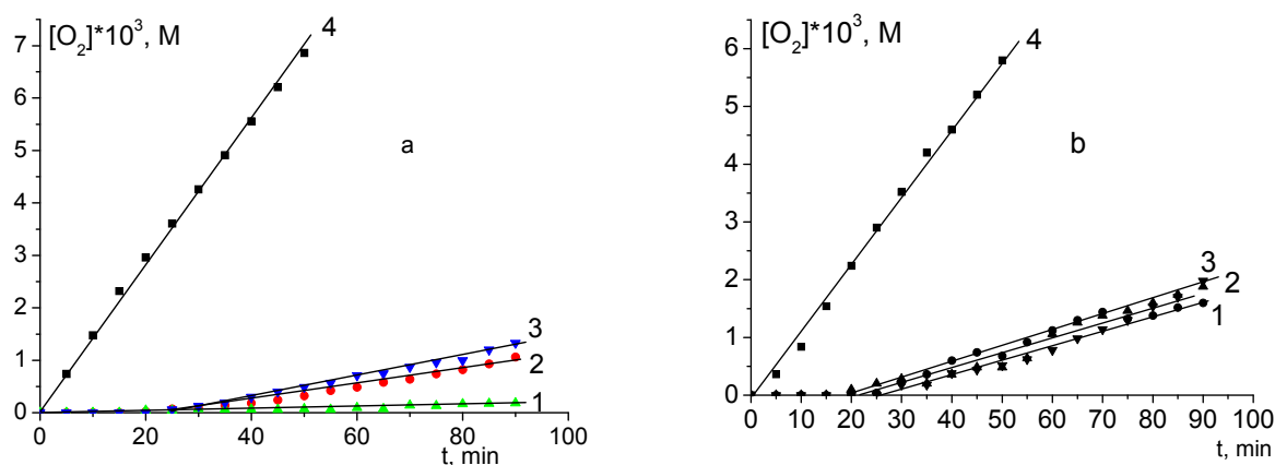
Figure 15. Effect of 0.1 mM (1) adrenalin, (2) dopamine, (3) noradrenalin on AAPH-initiated (55 mM) oxidation of PL (45 mg/ml) at 37^\circ C in (a) water and (b) in phosphate buffer with pH 7.4; (4) no additives.
