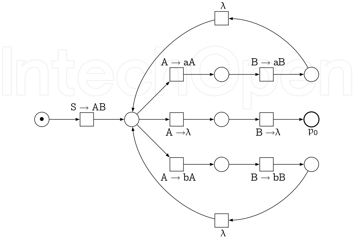
Figure 4. A labeled state machine N_4
