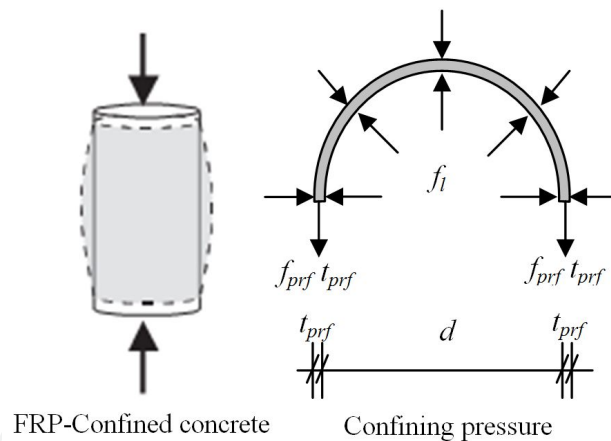
Figure 1. Confinement action of FRP jacket in circular sections
