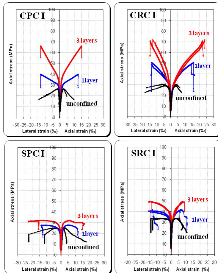
Figure 8. Experimental stress strain curves of normal-strength concrete specimens (26 MPa)
