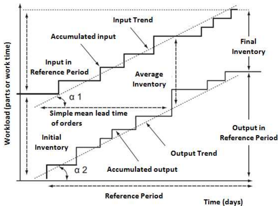
Figure 2. Throughput diagram of a work center
