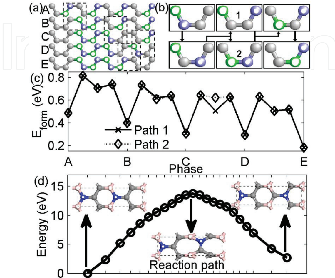
Figure 2. (a) Different steps (A-E) of phase separation process, (b) Swapping of BN and C dimers, (c) Formation energies for different steps shown in (a) for two different paths demonstrated in (b), (d) Activation energy in going from left to right configuration in the initial step of phase segregation. Reprinted with permission from Appl. Phys. Lett. 98, 022101 (2011). Copyright (2011) American Institute of Physics.
