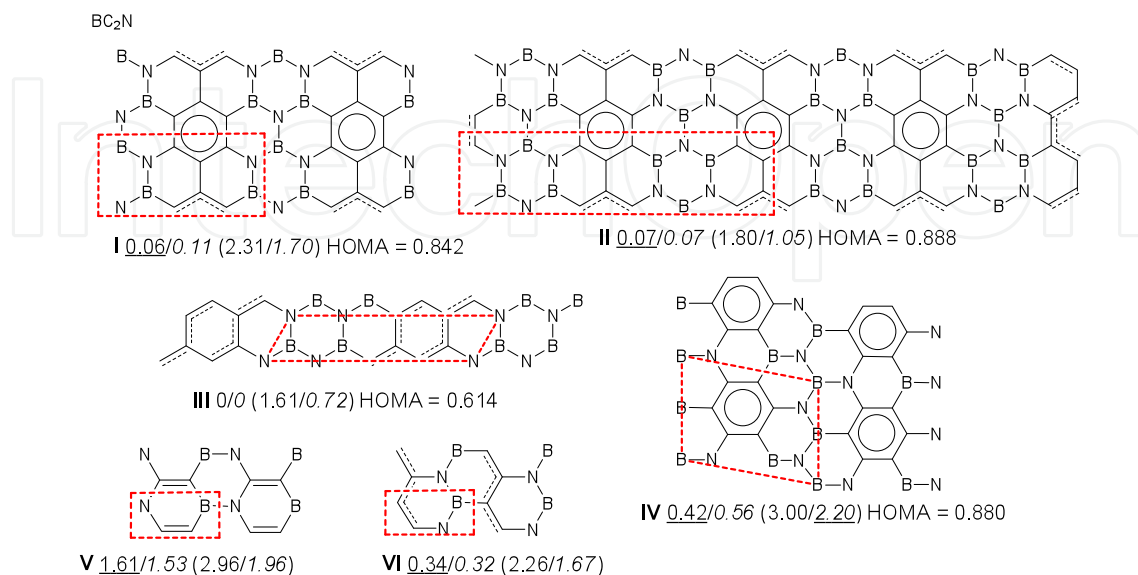
Figure 5. Six isomers of BC 2 N are considered for this study. Relative energy (per formula unit) with respect to most stable structures and band gaps (in parentheses) are shown from HSE (normal print) and PBE (italic) calculations. HOMA values of all-C hexagons, obtained from HSE calculations are also provided. Reprinted with permission from J. Phys. Chem. C 115, 10264 (2011). Copyright (2011) American Chemical Society.
