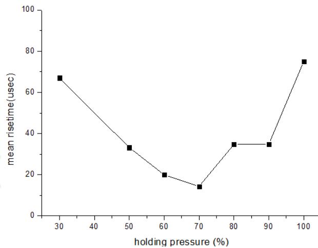
Figure 7. Mean rise time during load holding
