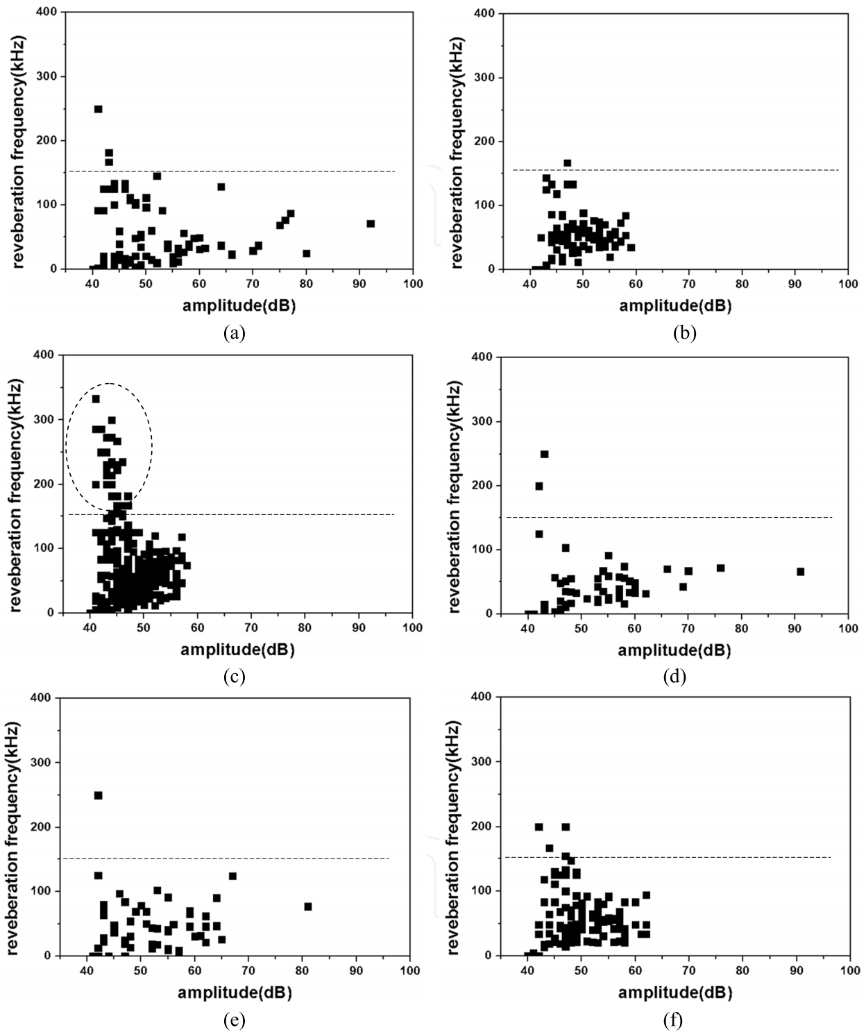
Figure 33. The reverberation frequency distribution of hits connected with event during fatigue cycle for longitudinal defect vessel: a) 0, b) 4000, c) 8000, d) 12000, e) 16000, f) 20000 cycles
