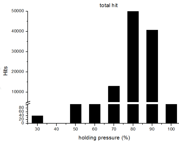
Figure 6. Total hits during load holding
