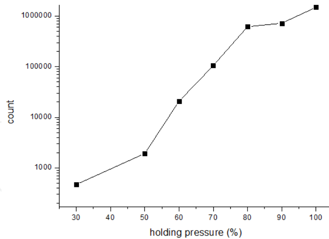
Figure 11. Total count during load holding
