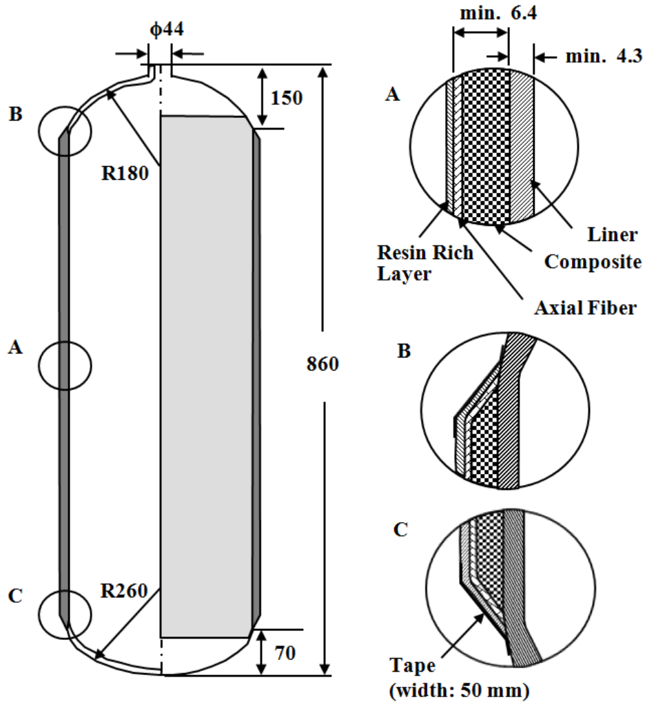
Figure 1. Schematic diagram of experimental vessel
