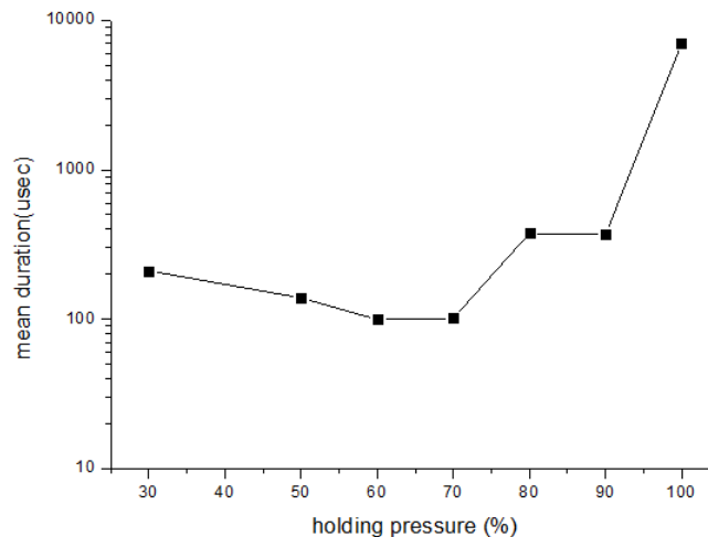
Figure 8. Mean duration during load holding
