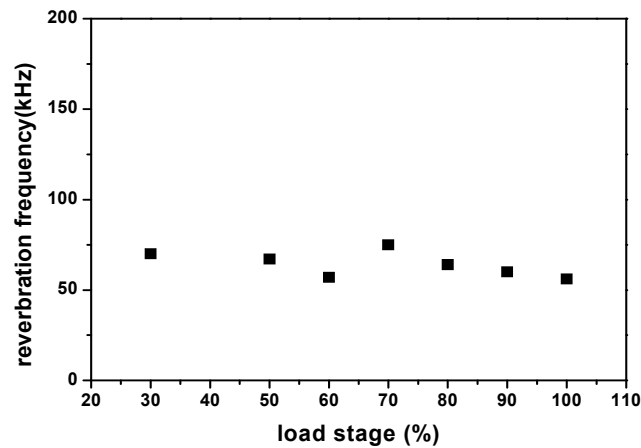
Figure 20. Mean reverberation frequency during each loading stage
