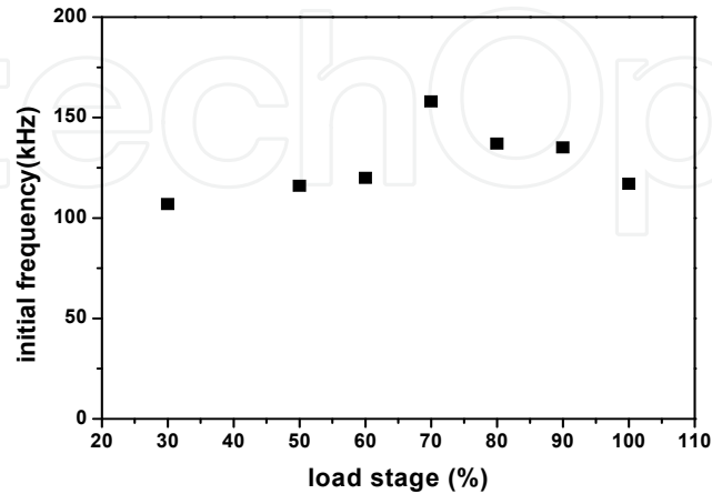
Figure 19. Mean initial frequency during each loading stage
