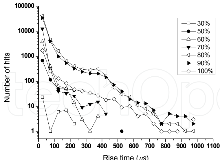
Figure 16. Rise time distribution during load holding
