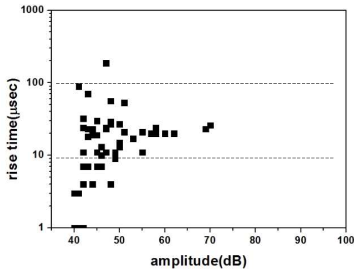
Figure 36. Distribution of rise time on the amplitude of the signals
