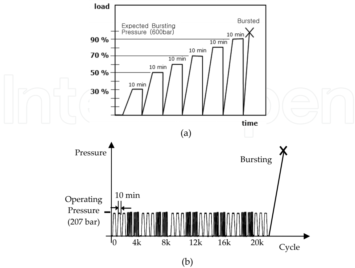
Figure 3. Loading sequence : (a) Burst and (b) fatigue test
