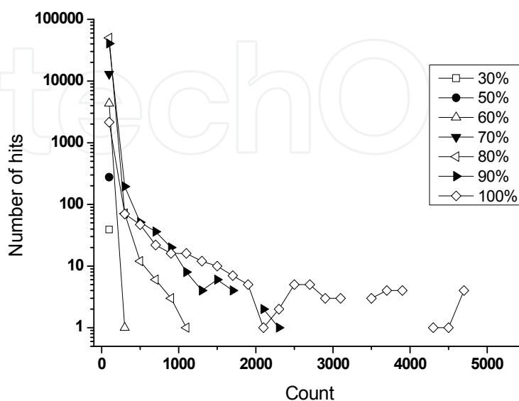
Figure 14. Count distribution during load holding
