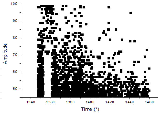
Figure 5. Amplitude vs Time plot during load holding : (a)30% (b)50% (c)60% (d)70% (e)80% (f)90% and (g)fractured
