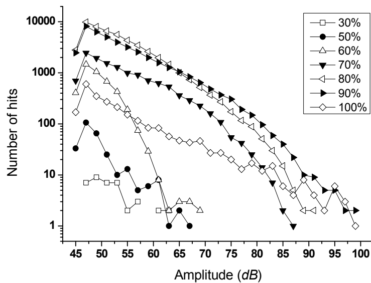
Figure 13. Amplitude distribution during load holding
