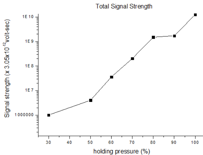
Figure 12. Total signal strength during load holding
