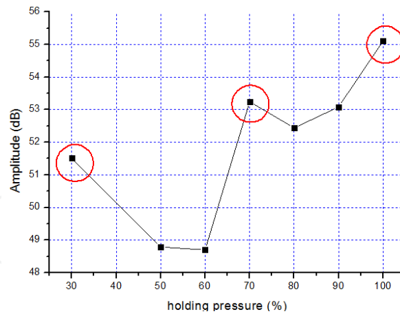
Figure 9. Mean amplitude during load holding
