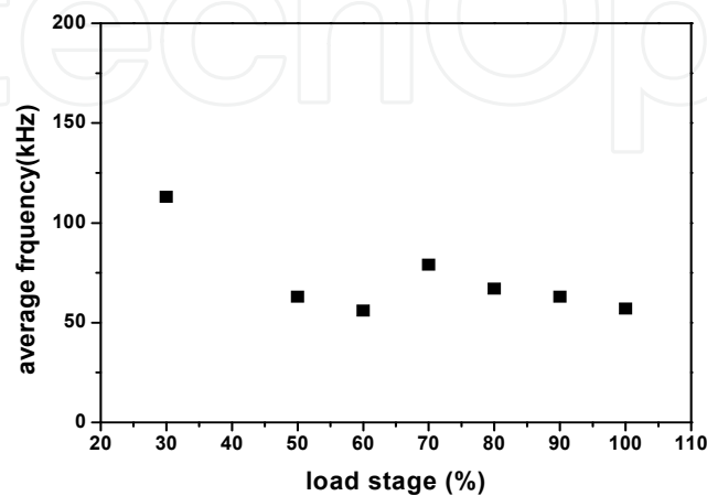
Figure 21. Mean average frequency during each loading stage
