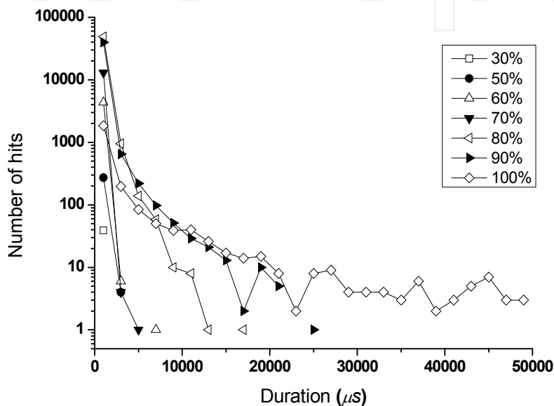
Figure 15. Duration distribution during load holding
