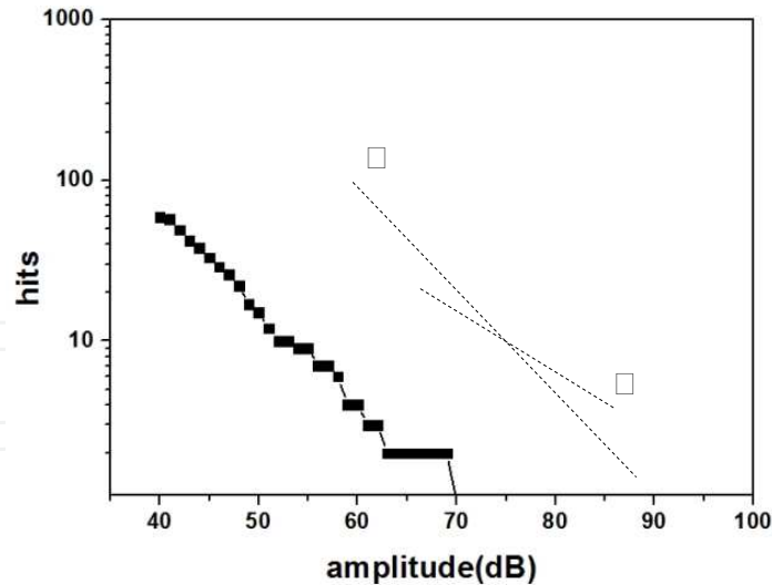
Figure 35. The amplitude distribution of accumulated hits connected with event during fatigue cycle for longitudinal defect vessel
