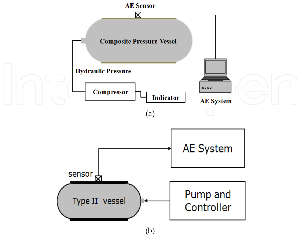
Figure 2. Diagram of Experimentation : (a) Burst and (b) fatigue test of the composite vessel
