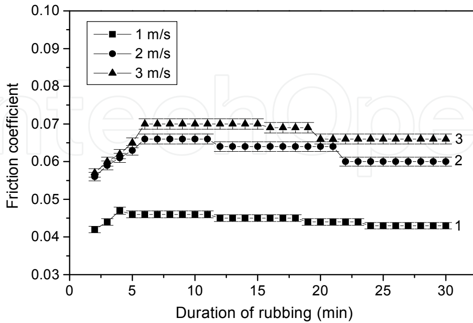
Figure 6. Friction coefficient as a function of duration of rubbing at different sliding speeds, normal load: 15 N, relative humidity: 70%, test sample: glass fiber.
