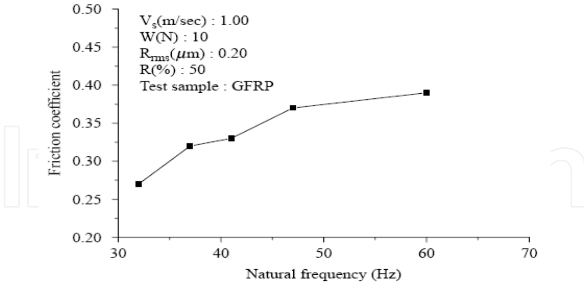
Figure 34. Variation of friction coefficient with the variation of natural frequency of the experimental set-up for GFRP
