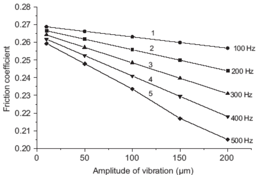
Figure 18. Variation of friction coefficient with the variation of amplitude of vibration at different frequency of vibration (sliding velocity: 1.17 m/s, normal load: 10 N, roughness: 0.2 \mu\text{m} (RMS), relative humidity: 50%, test sample: glass fiber reinforced plastic).
