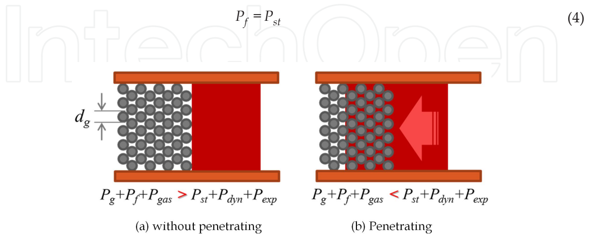
Figure 8. Pressure balance and penetration defect.
