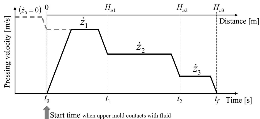
Figure 4. Pressing input shaped by trapezoidal velocities.
