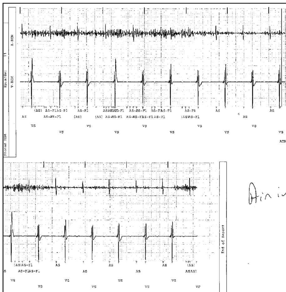
Figure 10. Noise caused by air in header. Atrial electrogram during device interrogation revealed high-frequency noise during sinus rhythm. This patient was not pacemaker dependent so there was no failure to pace.
