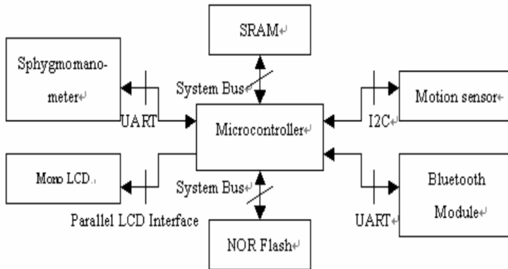
Figure 7. Wristable sphygmomanometer hardware architecture
