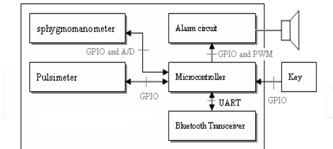
Figure 6. Wristable sphygmomanometer and pulsimeter hardware architecture
