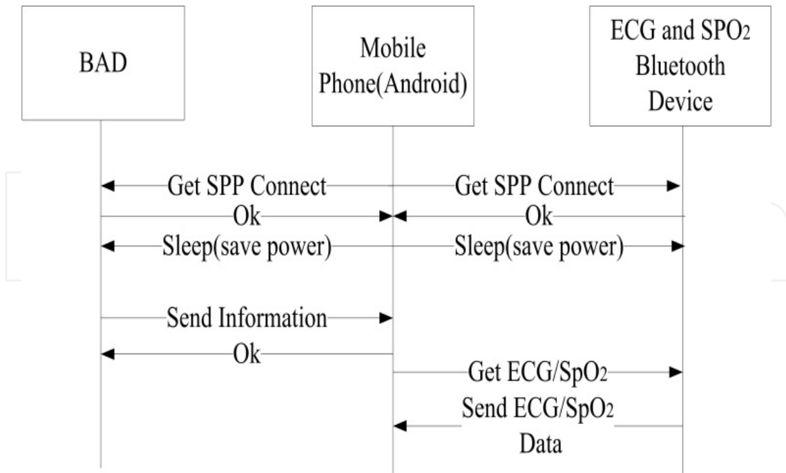
Figure 22. System communication
