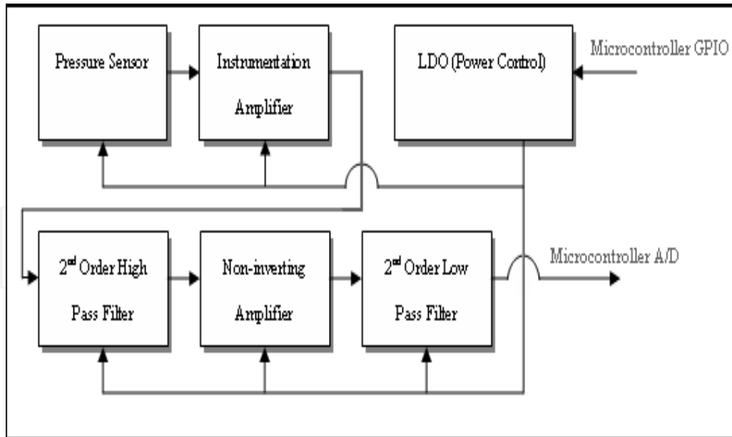
Figure 8. Sphygmomanometer device
