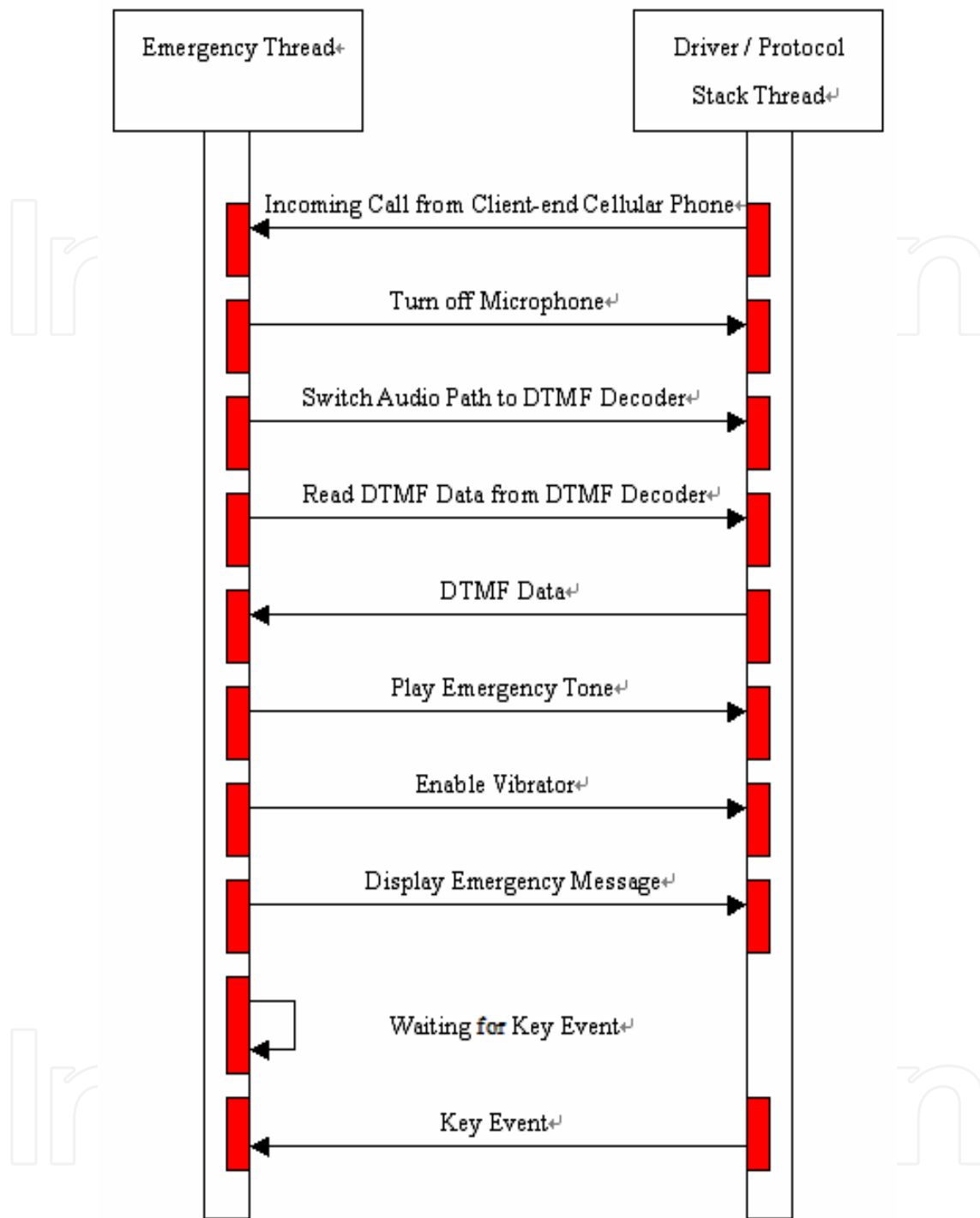
Figure 20. Emergency procedure of the server-end cellular phone of tele-emergency announcement system
