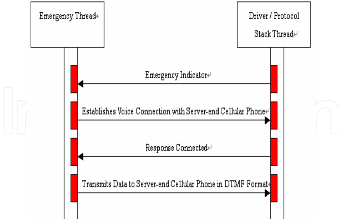
Figure 19. Emergency procedure of the wristable sphygmomanometer of the tele-emergency announcement system
