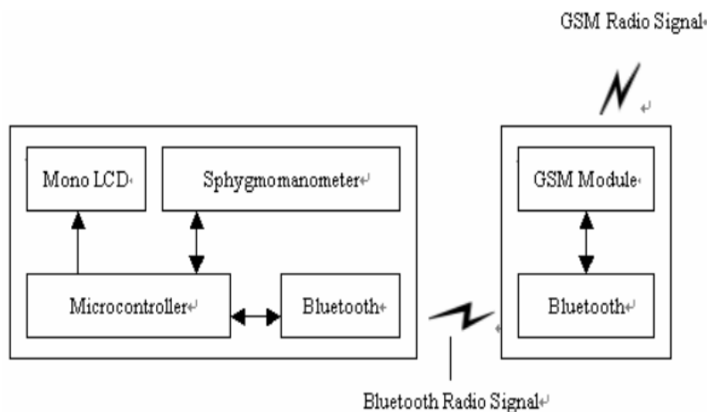
Figure 4. Tele-care system architecture
