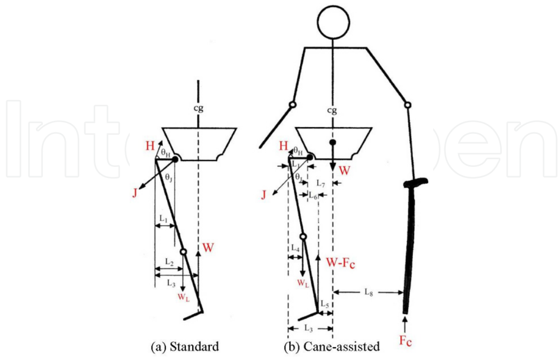
Figure 6. Diagram for boundary conditions of cane-assisted walk.
