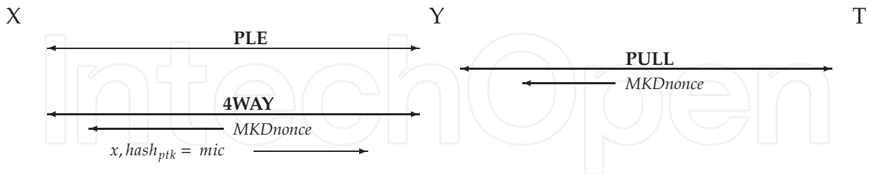
Figure 8. MSA Authentication. The text above a double-headed arrow (e.g., 4WAY ) is a protocol, and text below (e.g., MKDnonce ) is some data that is sent as part of the protocol.
