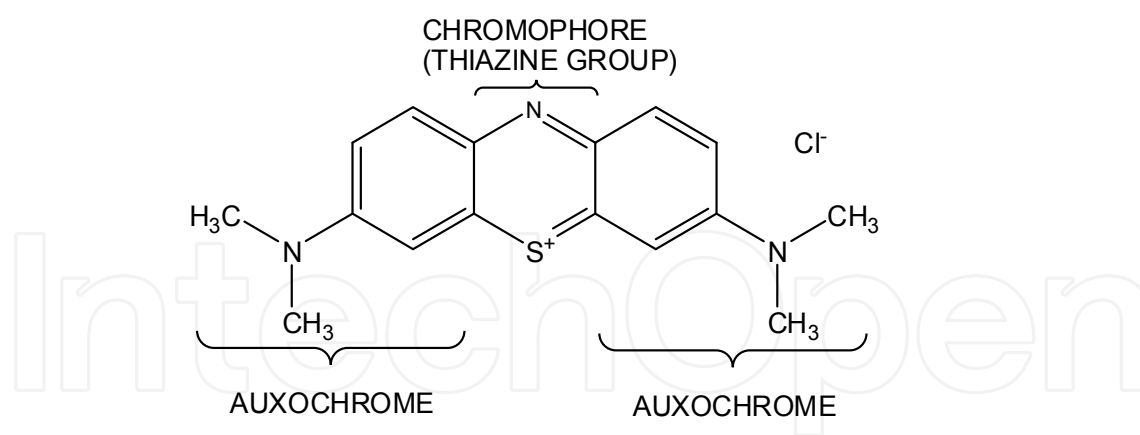
Figure 13. Example of the presence of chromophores and auxochromes in basic blue 9.
