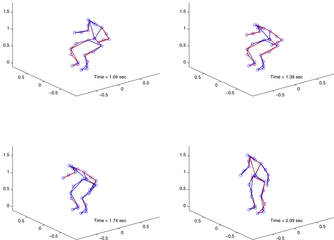
Figure 5. Fast STS: kinematic fit for four time instant t_k ; superimposition of the fitted model coordinates x_{exp,n}(t_k) (in blue) and the experimental model coordinates x_{mod,n}(q(t_k)) (in red).
