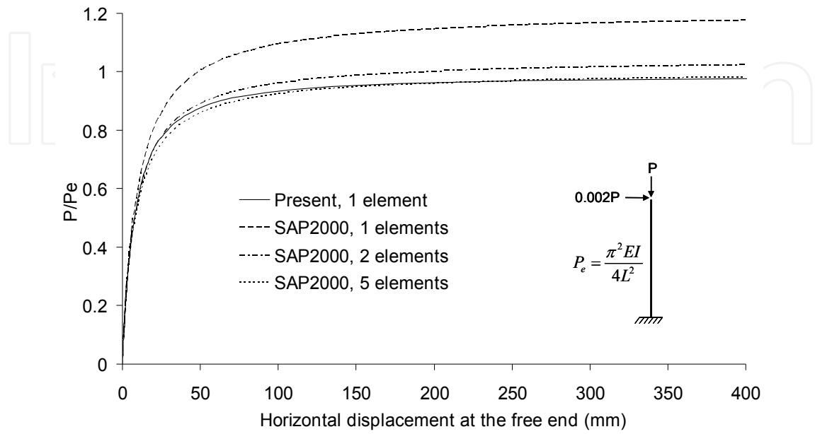
(a) Cantilever column
