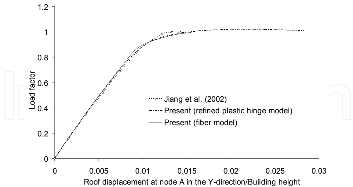
Figure 16. Load-displacement curves of twenty-story space frame
