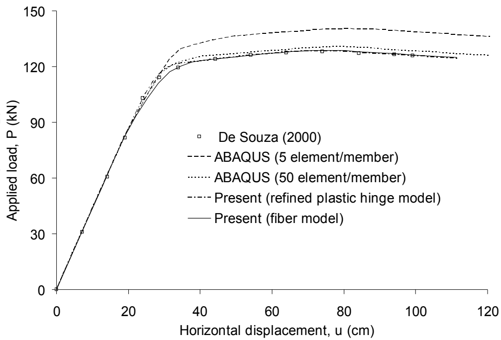
Figure 14. Load-displacement curves of two-story space frame
