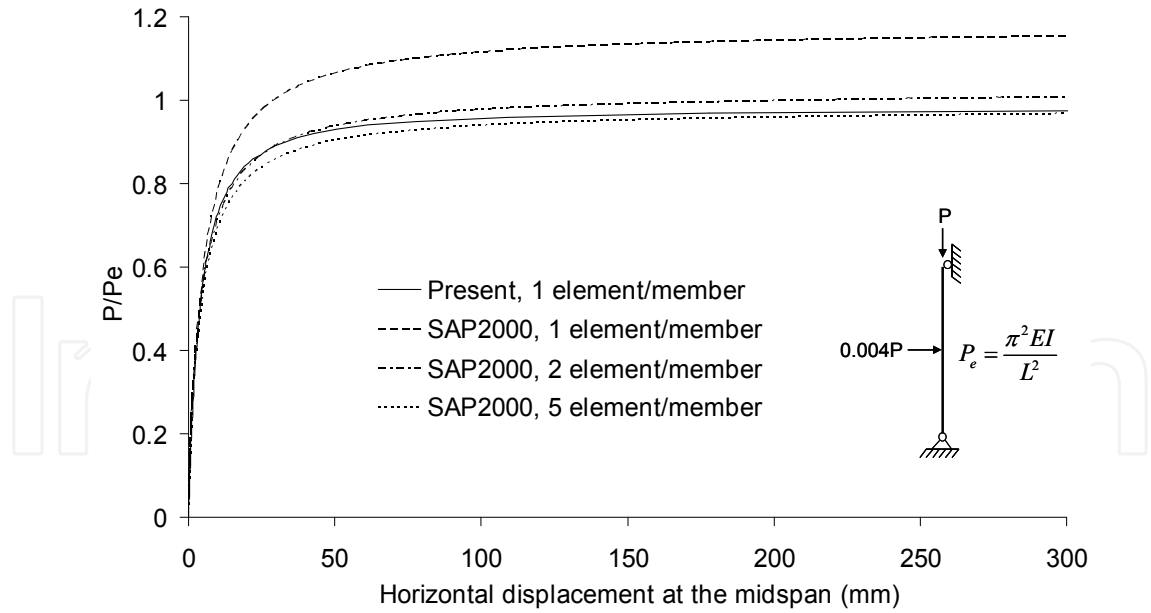
(b) Simply supported column
