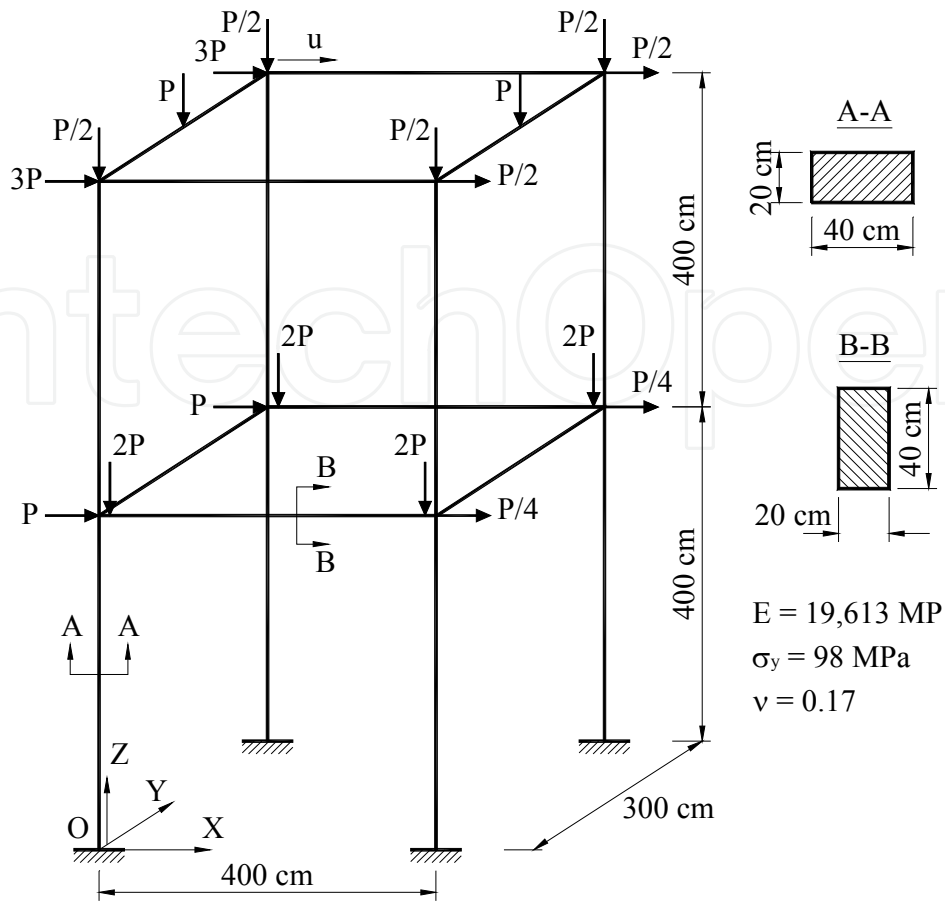
Figure 13. Two-story space frame
