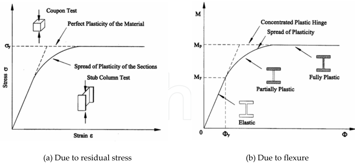
Figure 4. Gradual yielding of steel member
