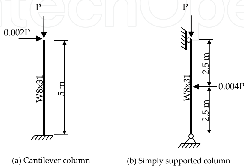
Figure 11. Steel columns
