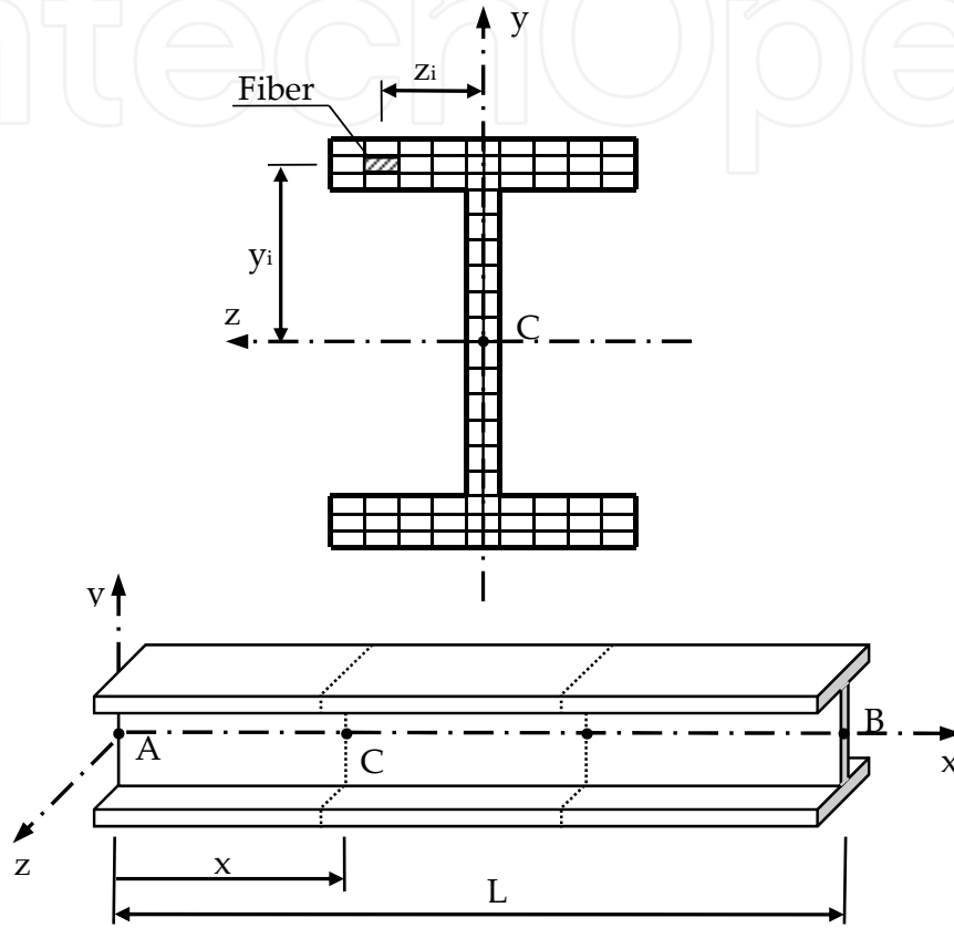
Figure 9. Fiber hinge model
