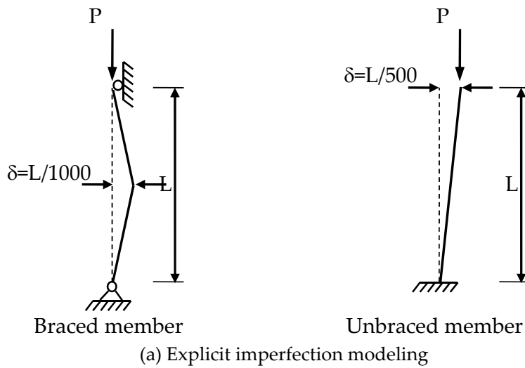
Figure 1. The P - \delta and P - \Delta effects of a beam-column
