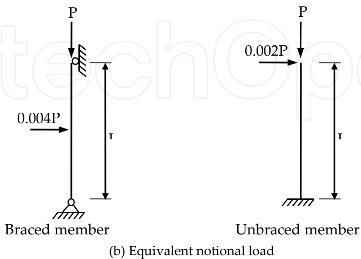
Figure 2. Geometric imperfection methods
