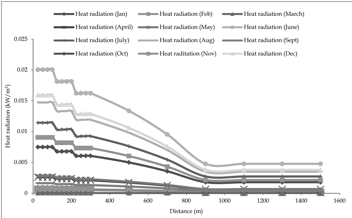
Figure 4. Heat radiation from gas flaring (Station 1) with a stack efficiency of 75%
