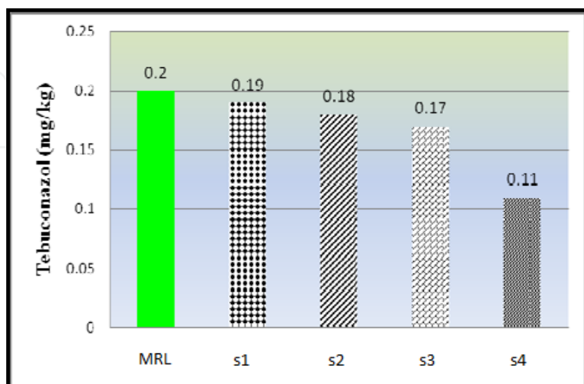
Figure 3. Tebuconazol content compared with MRL
