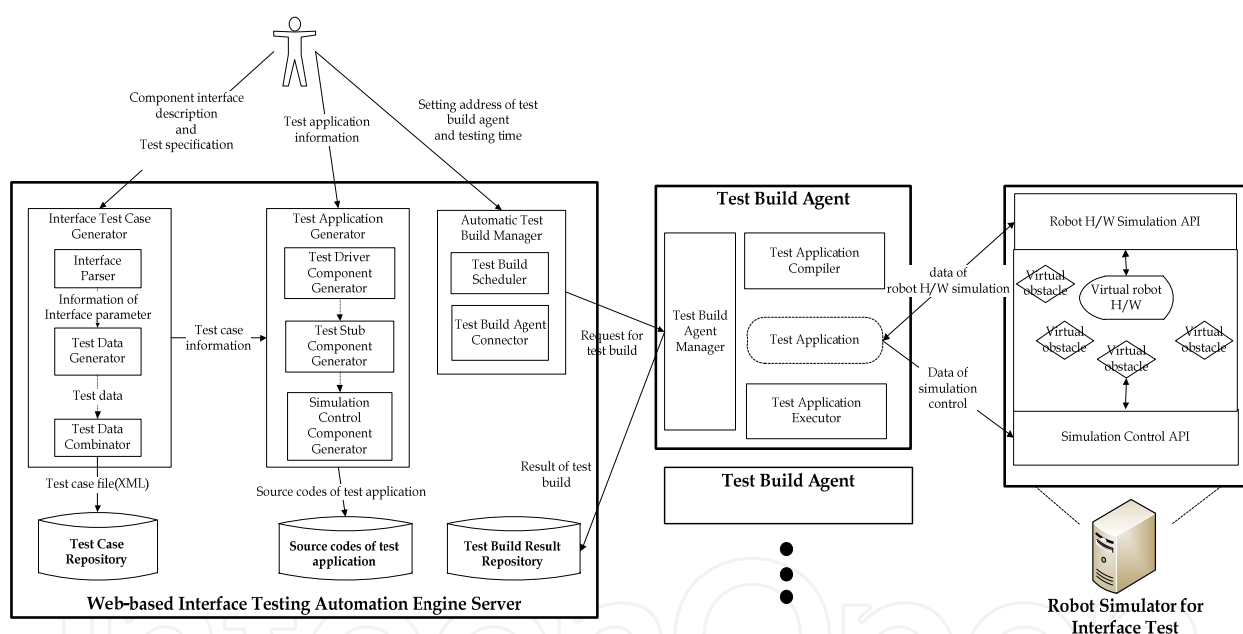
Fig. 1. Simulation-based Interface Testing Automation Framework Architecture
