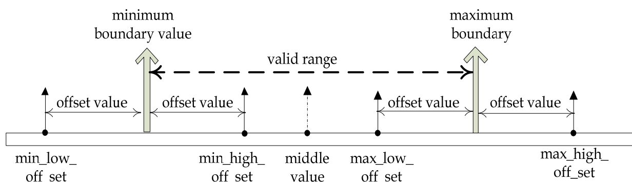
Fig. 6. Offset and test data of BVA scheme
