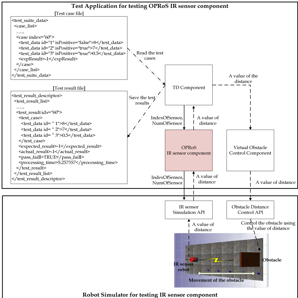
Fig. 12. Application for testing the IR component interface
