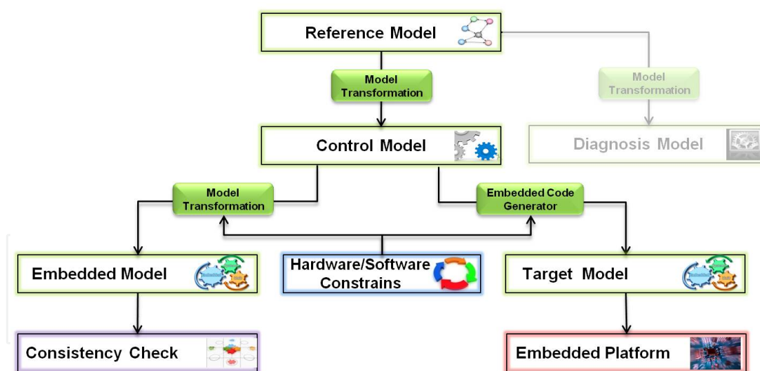
Fig. 1. Framework Overview
