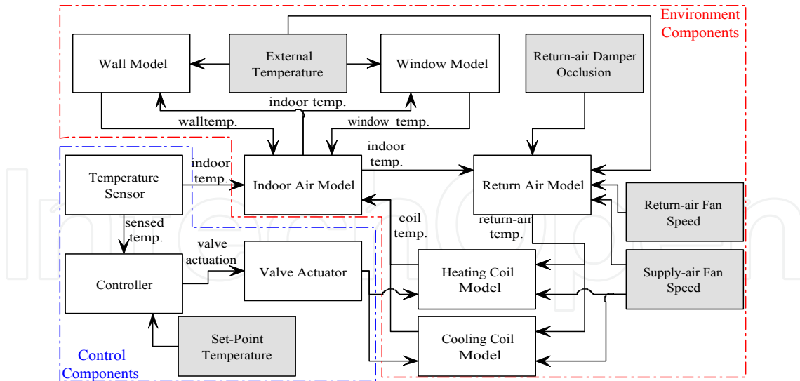
Fig. 11. AHU Component-Based Model
