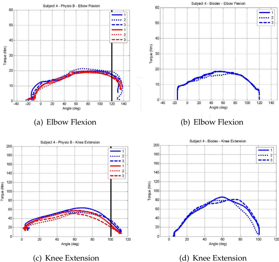
Fig. 4. Strength profiles of one participant for concentric elbow flexion and knee extension obtained from the IRL-HHD (a, c) and the Biodex (b, d).
