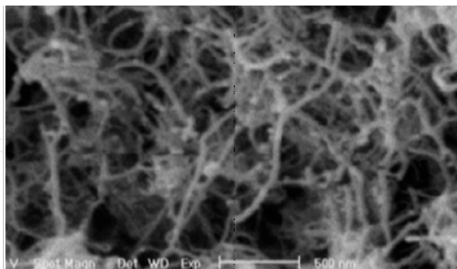
Figure 13. Production of CNTs in NaCl solution [62].
