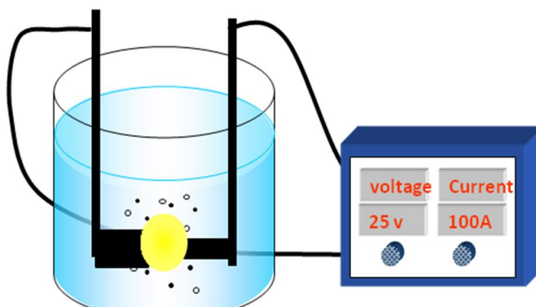
Figure 5. Schematic device of arc discharge in liquid.
