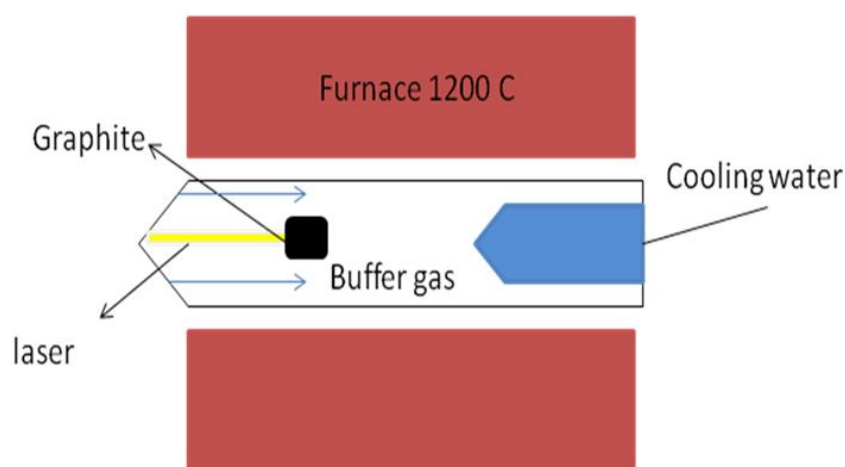
Figure 1. Schematic drawing of a laser obtain.
