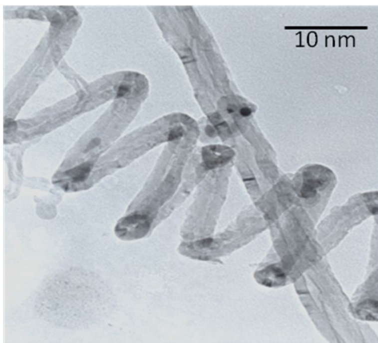
Figure 4. Carbon nanotubes produced in LiCl 0.25 N [51].
