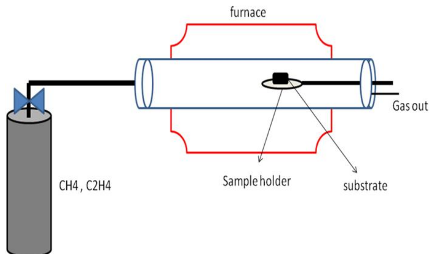
Figure 2. Schematic diagram of a CVD setup.
