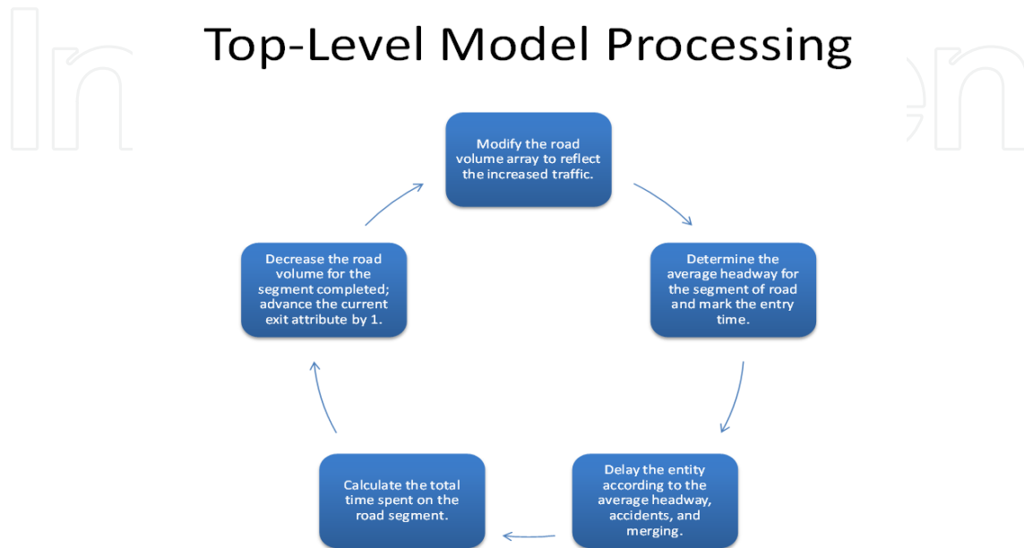
Figure 5. Transaction processing in the top-level model
