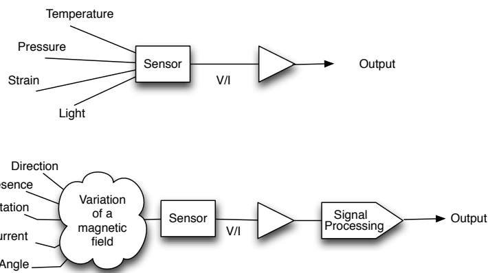
Figure 8. Difference between conventional sensors and magnetic sensors
