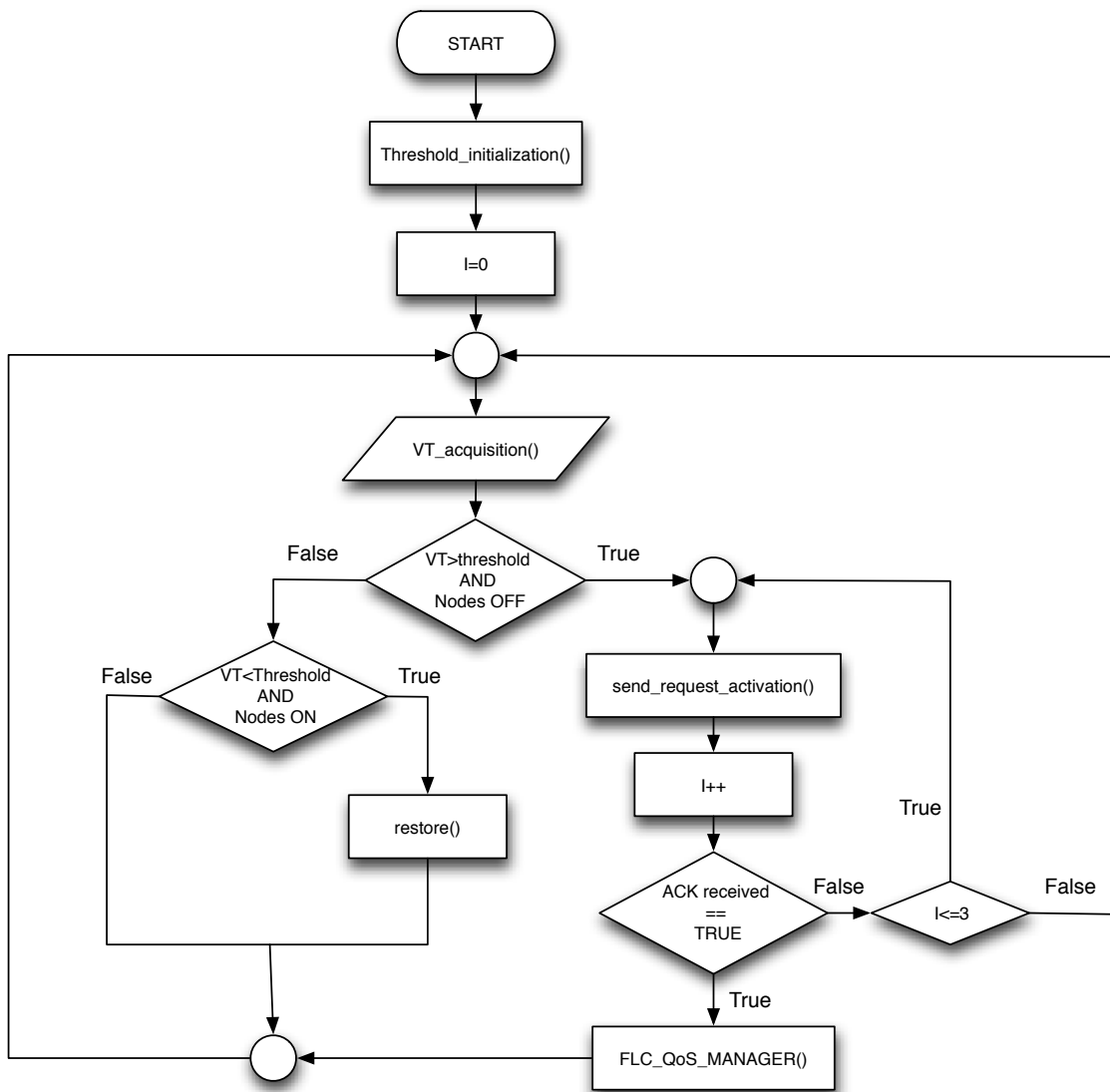
Figure 15. DVMA flow chart
