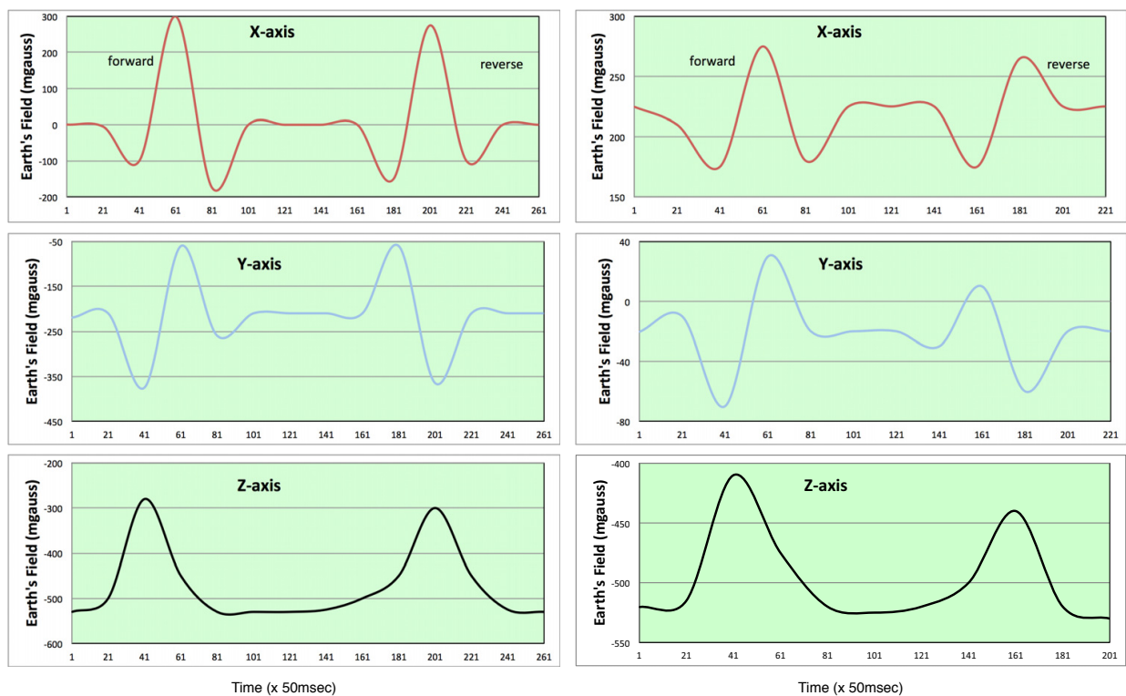
Figure 13. Direction Control
