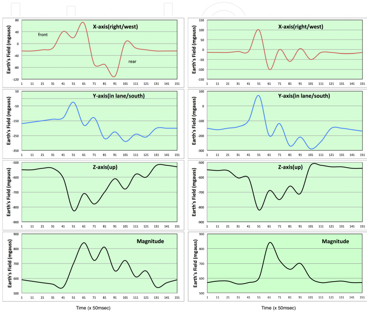
Figure 11. Vehicle classification
