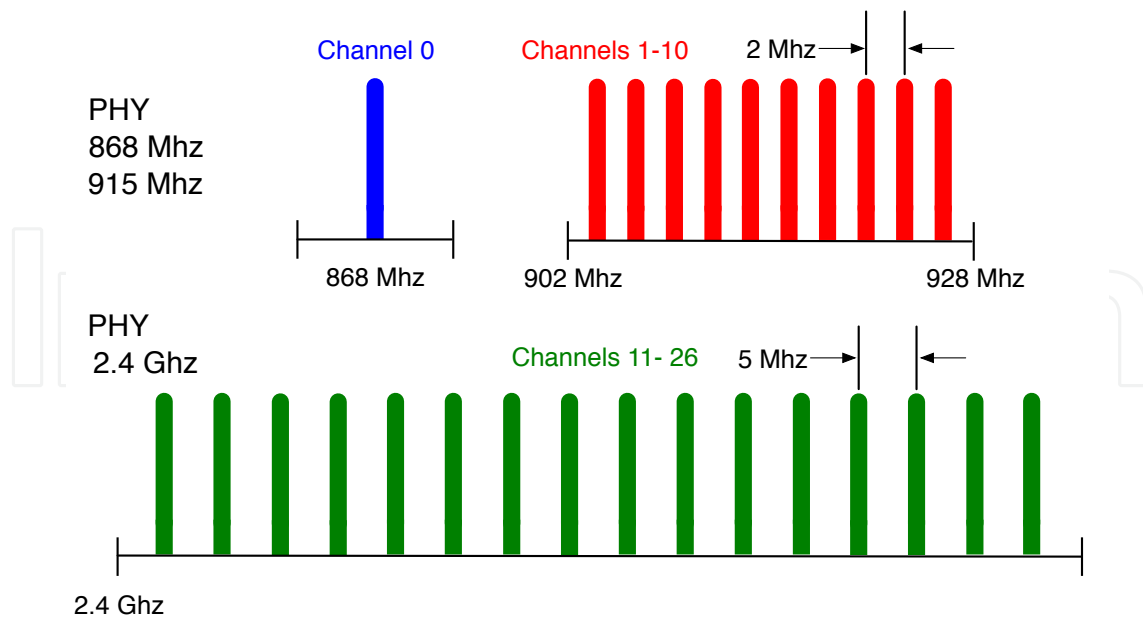
Figure 2. Physical layer
