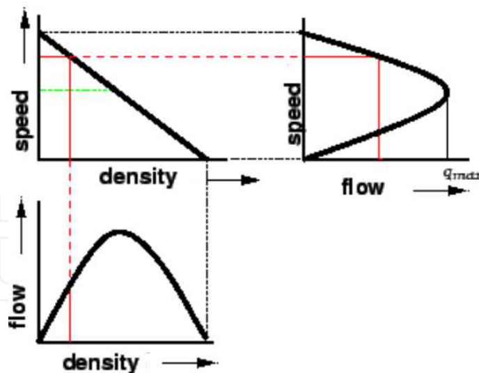
Figure 7. All Traffic Fundamental Relations
