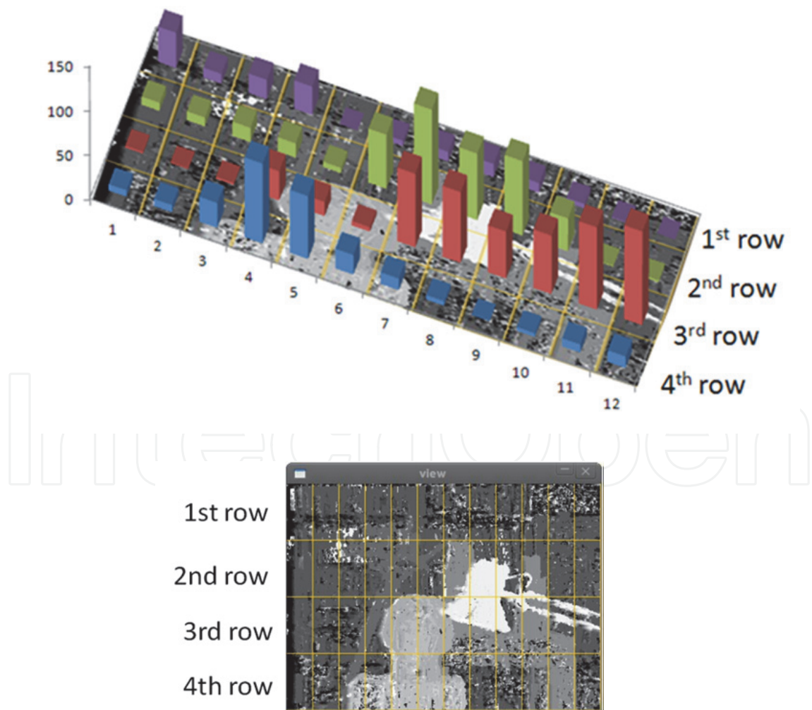
Figure 13. Depth map and 2D map of the Tsukuba images.
