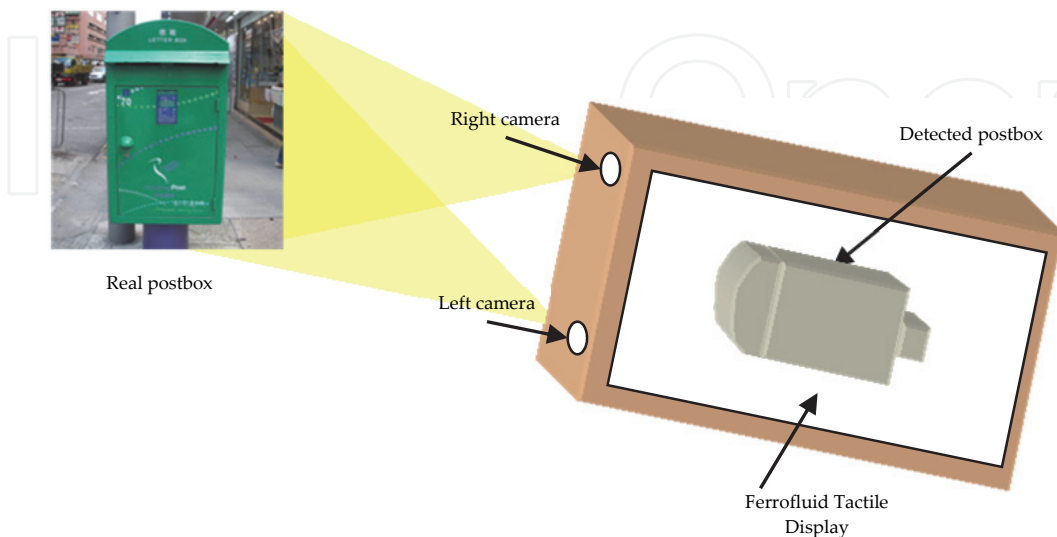
Figure 18. Prototype of Mobile 3D environment detector for Blind People
