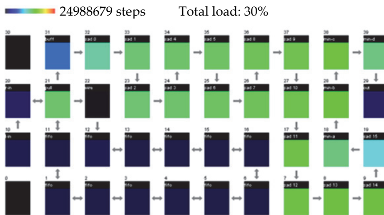
Figure 6. Heatmap of the developed SAD Algorithm.
