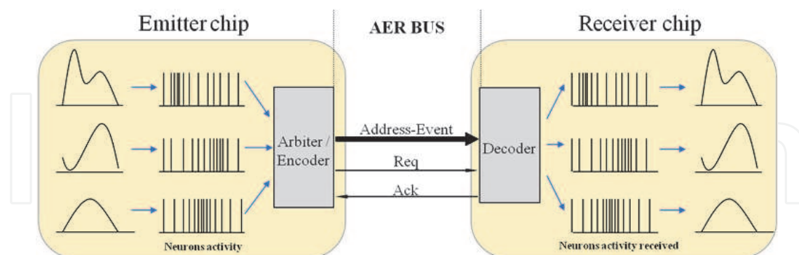
Figure 9. Rate-coded AER inter-chip communication scheme.
