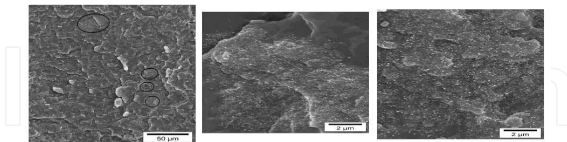
Figure 17. SEM micrographs of PP/PP-g-MWCNT composites with MWCNTs loading of 3wt%. Reproduced from [129] with permission of Elsevier.
