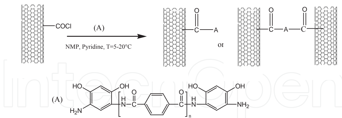
Figure 3. Synthesis of oligo-hydroxyamide-grafted MWNT. Reproduced from [80] with permission of Elsevier.
