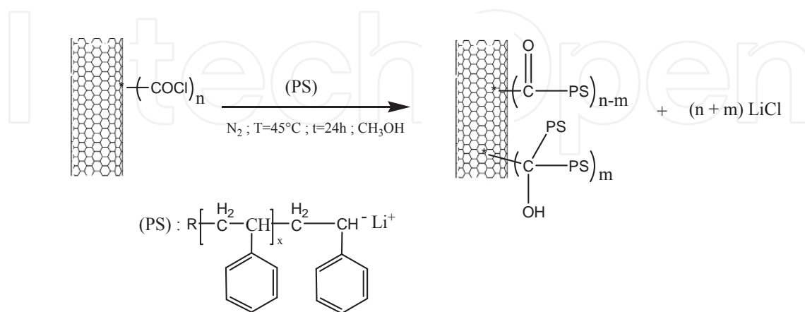
Figure 5. substitution reaction of living polystyryllithium anions with acyl chloride-modified CNTs. Reproduced from [86] with permission of John Wiley and Sons.
