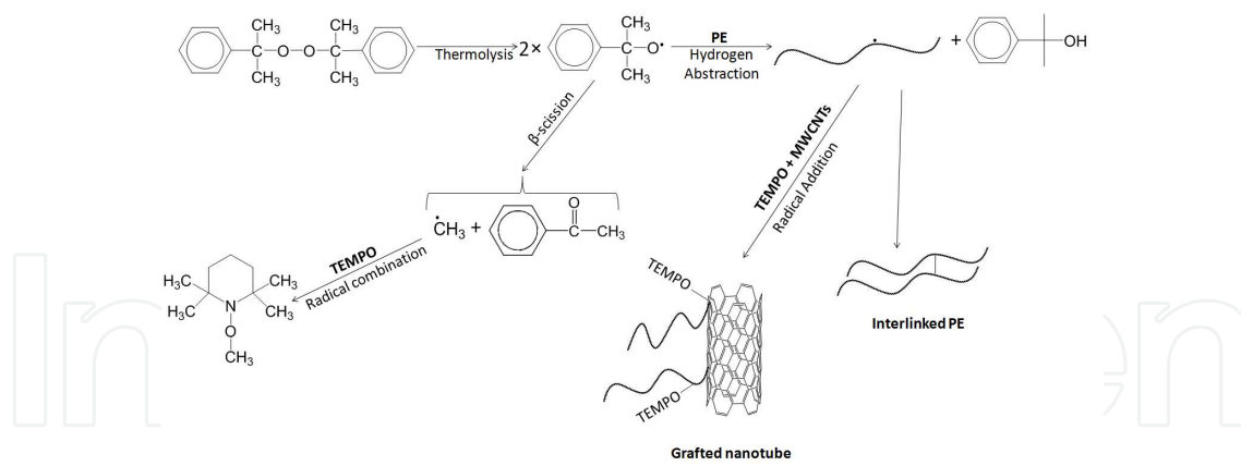
Figure 12. Reaction scheme for PE grafting onto MWCNTs with TEMPO as a radical scavenger. Reproduced from [128] with permission of John Wiley and Sons.
