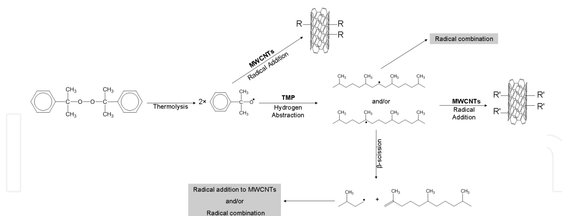
Figure 16. Reaction scheme for the addition of TMP onto CNT in the presence of DCP. Reproduced from [129] with permission of Elsevier.
