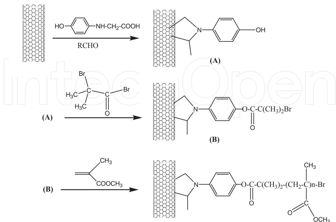
Figure 9. ATRP 'grafting from' modification approach. Reproduced from [92] with permission of ACS publications.
