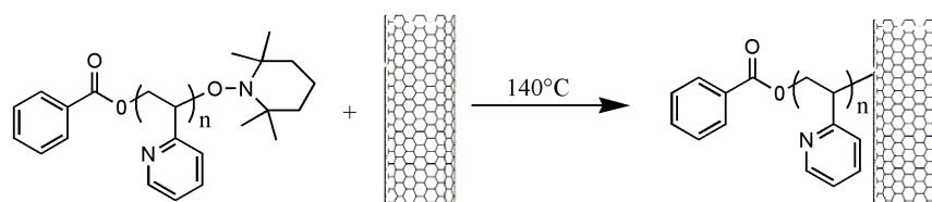
Figure 6. Radical grafting of TEMPO-end capped PVP to MWCNTs. Reproduced from [87] with permission of Elsevier.
