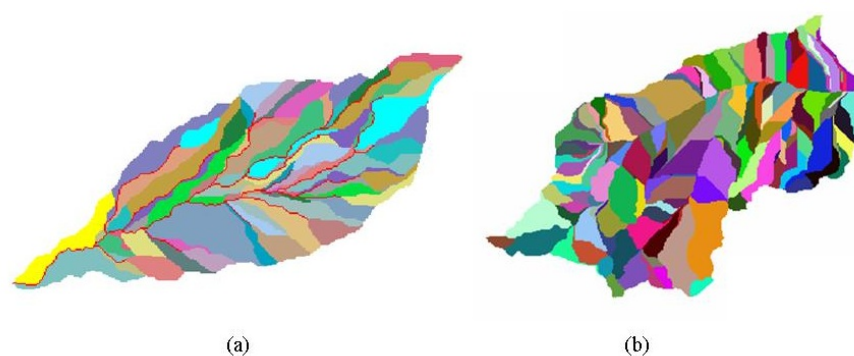
Figure 4. Layouts of the Cannata (left) and Ganspoel (right) watershed discretisation by the AnnAGNPS model.
