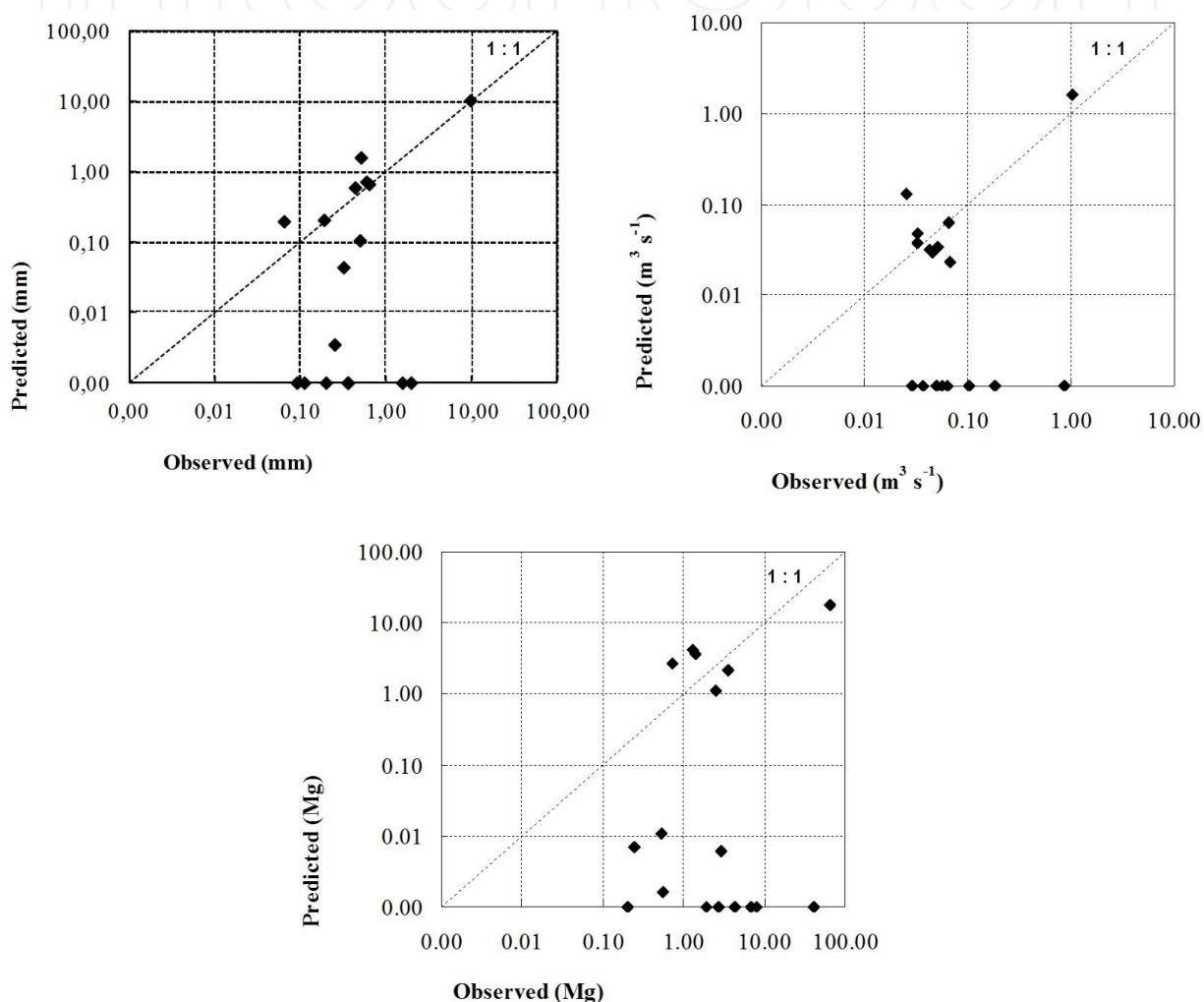
Figure 9. Comparison of 17 observed and simulated (by AnnAGNPS) events in the Ganspoel watershed, for runoff (upper left), peak flow (upper right) and sediment yield (bottom) (values are in logarithmic scale).
