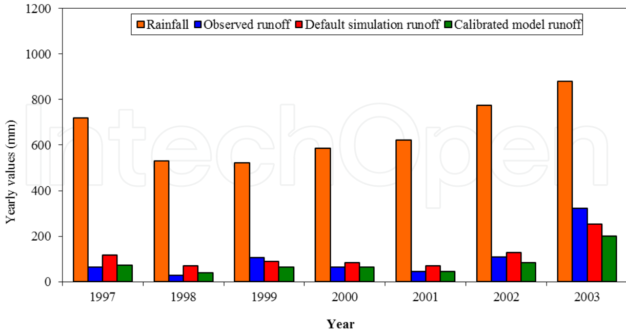
Figure 5. Comparison between observed and simulated (using default and calibrated parameters) yearly runoff volume for the years 1997 to 2003 at the Cannata watershed.
