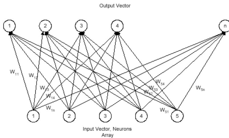
Figure 1. Topology Network of a SOM.
