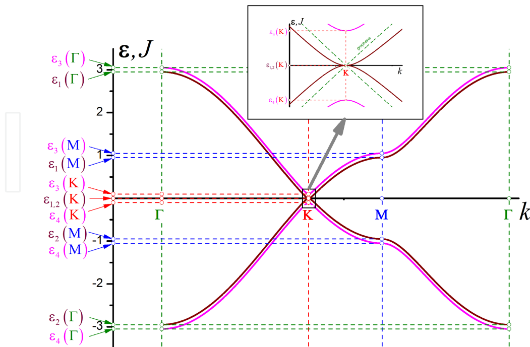
Figure 6. Dispersion curves along high-symmetry directions of bilayer graphene.
