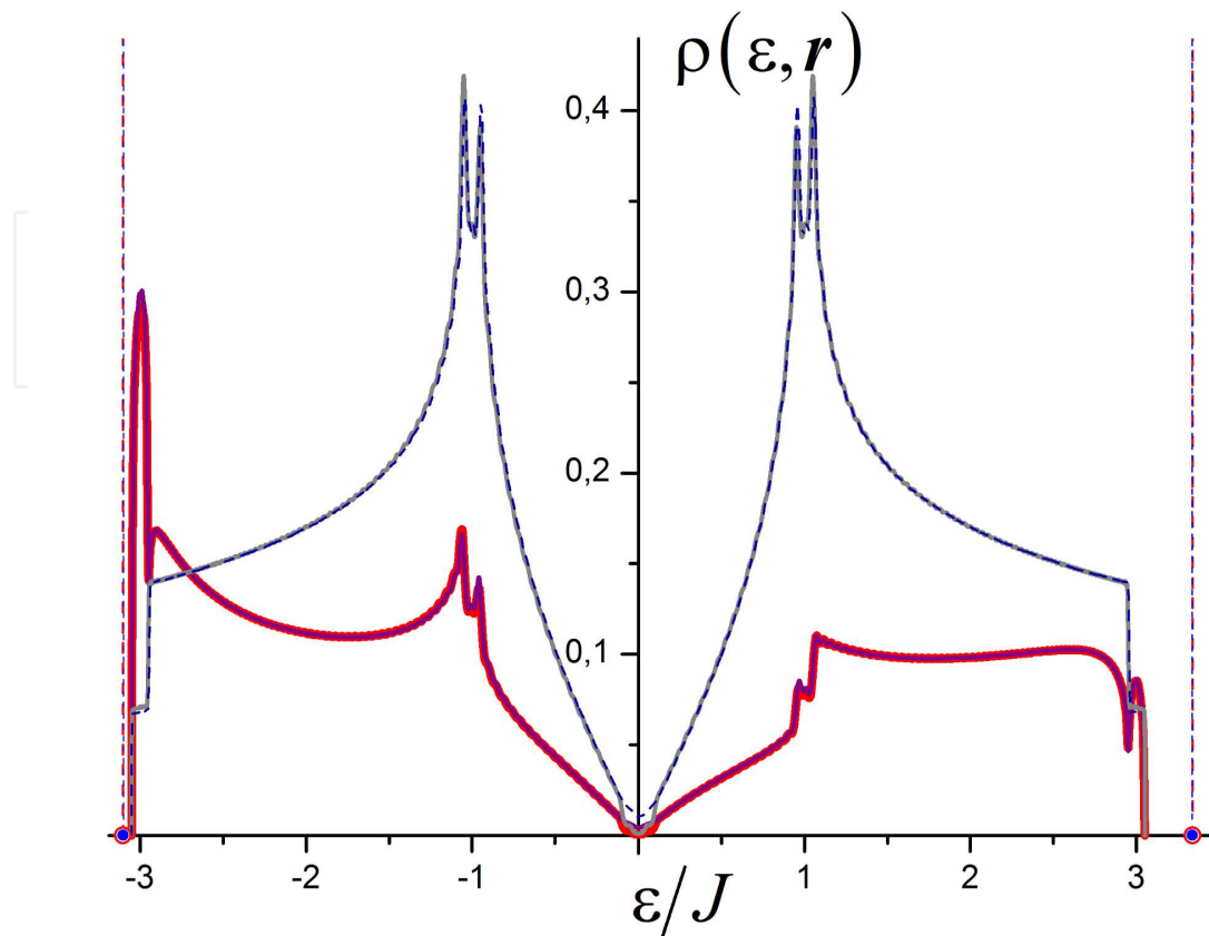
Figure 10. LDOS of the boron impurity in different sublattices of bigraphene (designations are the same as in Figure 9).
