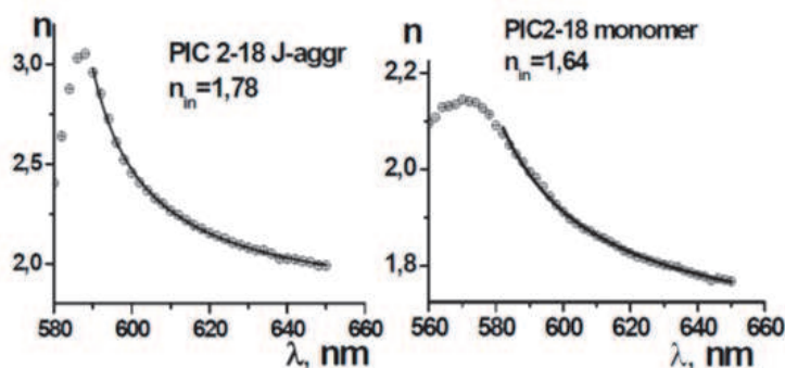
Fig. 13. Dispersion curves for PIC J-aggregate (a) and monomer (b) in the solid film (points) and their least square Zelmee approximation (line)
