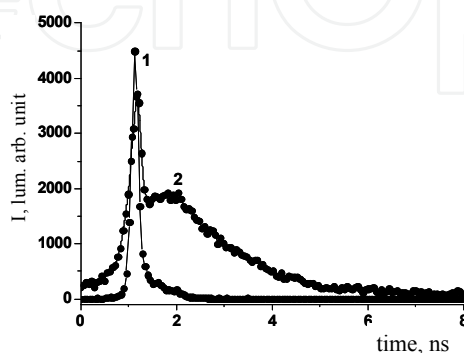
Fig. 30. Signal instrument function (1) and decay kinetics luminescence curve J-aggregates PIC2-15 in the film (2) excitation \lambda=574 nm measurement at 590 nm, T=96^{\circ}\text{K}
