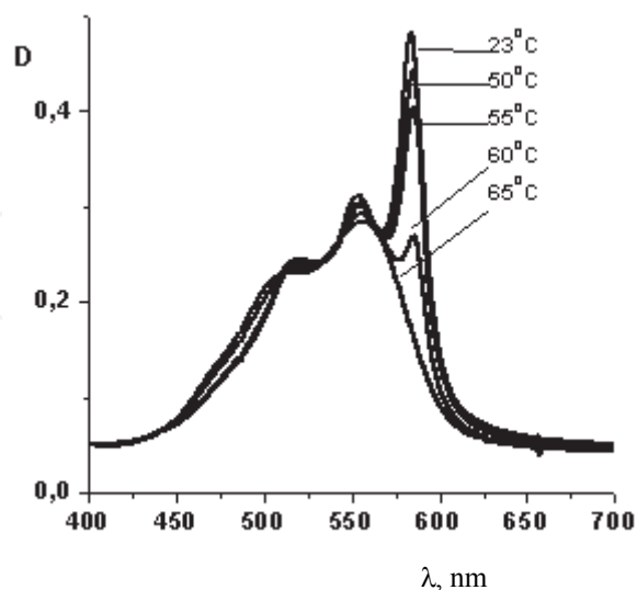
Fig. 3. The spectral change of the J-aggregated film PIC2-18 at sample heating
