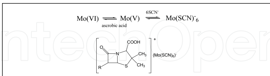
Fig. 14. Scheme of Mo(V)-thiocyanate- \beta -lactam ion-pair [48].
