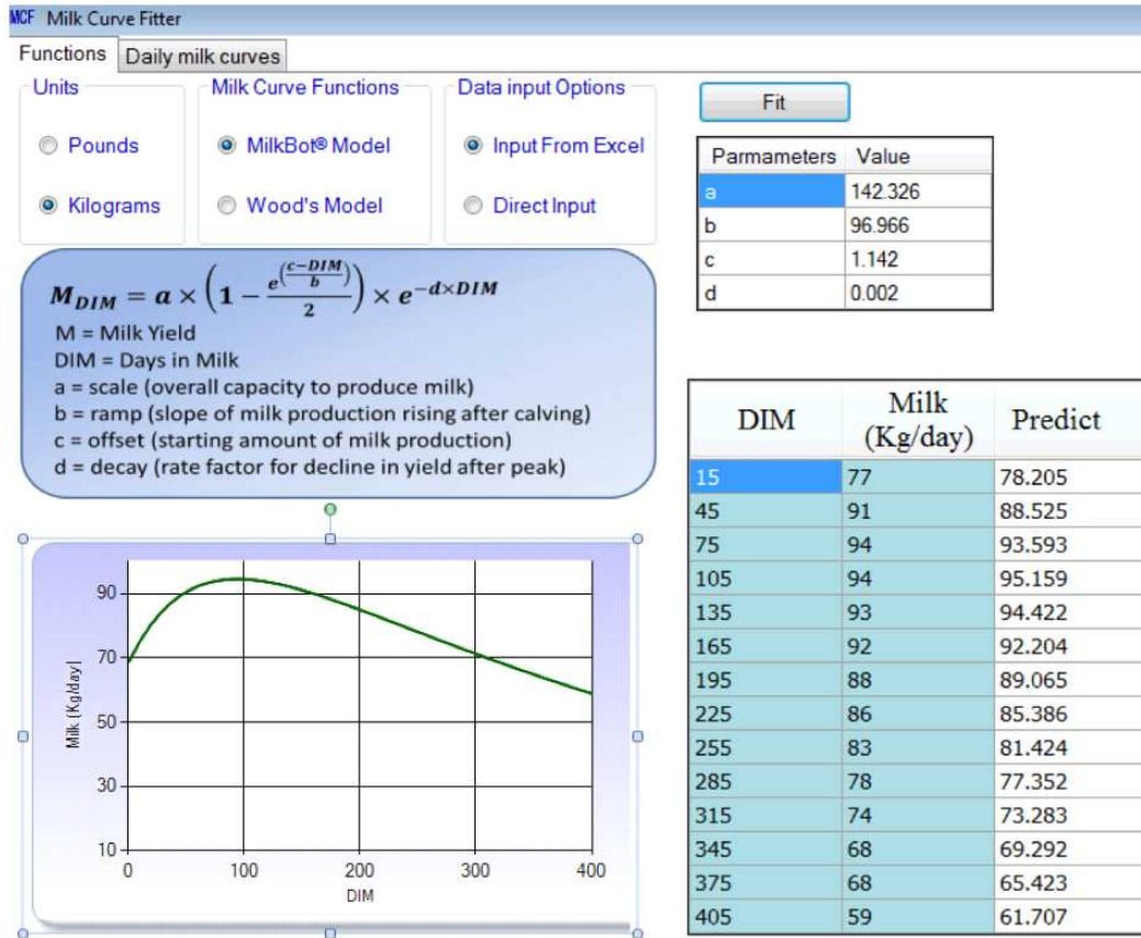
Figure 4. Screen snapshot of DSS Milk Curve Fitter.
