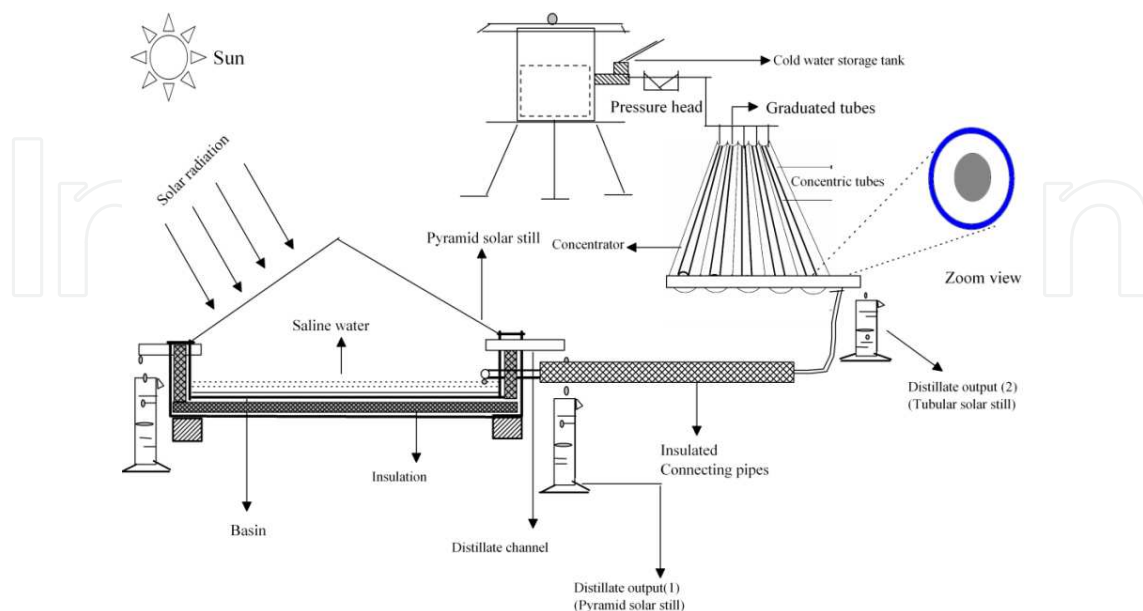
Figure 1. Cross sectional view of compound parabolic concnetrator tubular solar still coupled with pyramid solar still.
