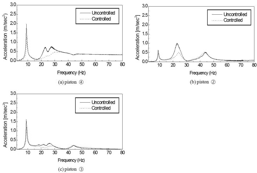
Figure 8. Acceleration response of the structural system with the MR mount.
