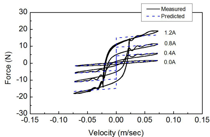
Figure 2. The field-dependent damping force of the MR mount.
