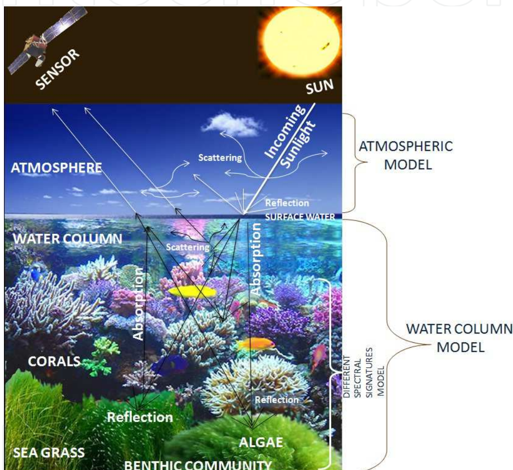
Fig. 1. Components of Remote Sensing in mapping coral reefs.
