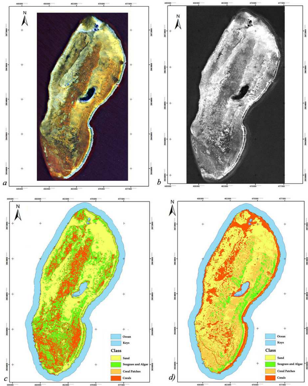
Fig. 8. a) Landsat 7-ETM+ image, RGB (1, 2, 3), b) image resulting from the depth-invariant index by bottom type using bands 1 and 2, and classification of the benthic bottom in the Chinchorro Bank using ISODATA, c) without water column correction and d) with water column correction.
