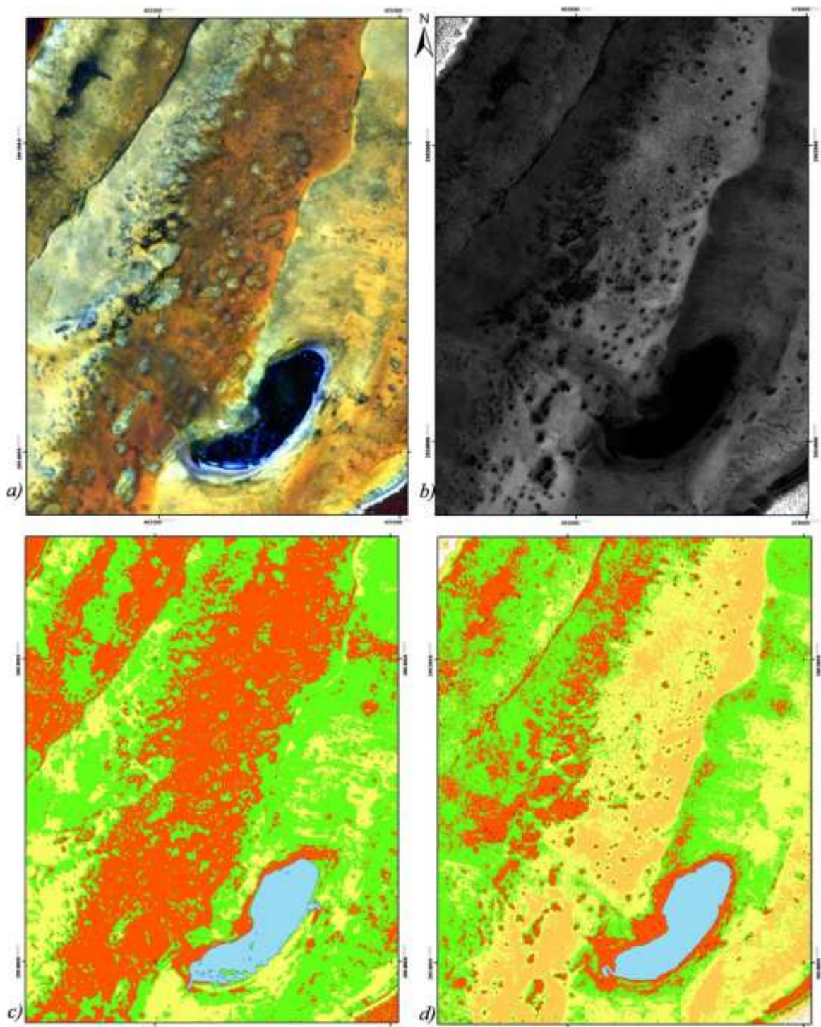
Fig. 9. Comparison among a) Landsat 7-ETM+ image, RGB (1, 2, 3), b) depth-invariant index by bottom type for bands 1/2, c) ISODATA without water column correction and d) ISODATA with water column correction.
