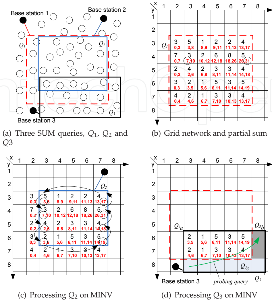
Fig. 3. Materialized in-network view
