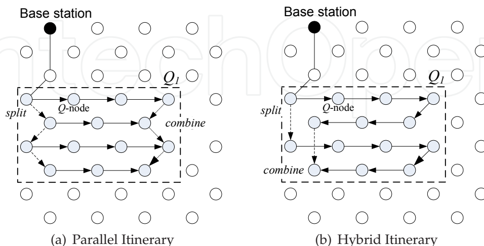
Fig. 2. Parallel and hybrid itinerary
