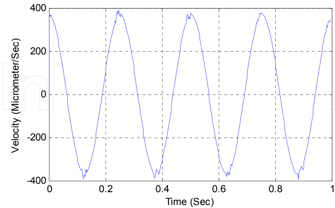
Fig. 3. Piezoelectric velocity.
