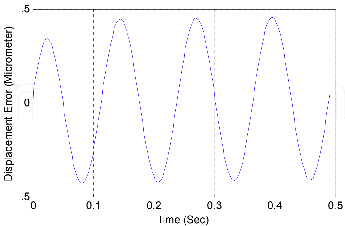
Fig. 10. Displacement Error of the method presented in [19].
