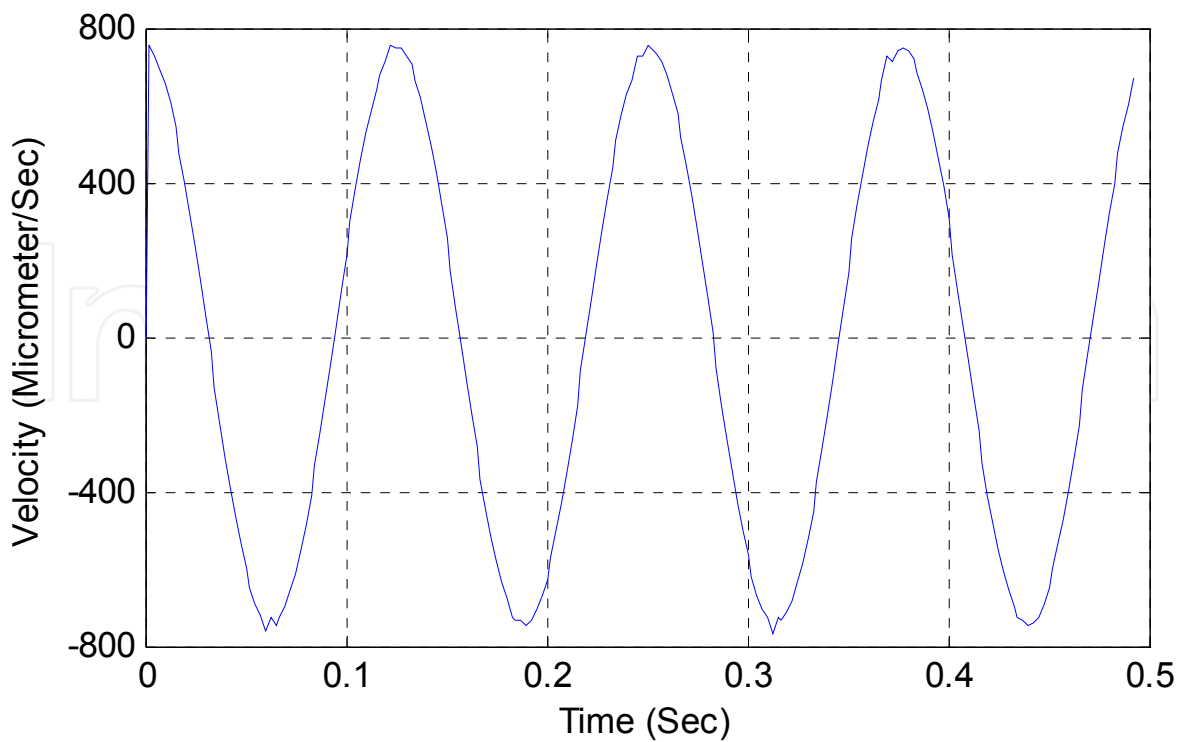
Fig. 6. Velocity of piezoelectric.
