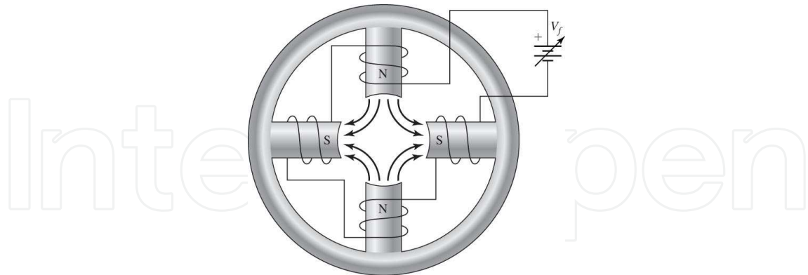
Fig. 5. Field coils and field poles of a dc machine
