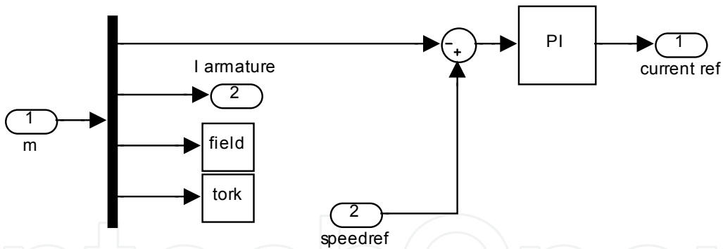
Fig. 13. Speed controller of dc machine
