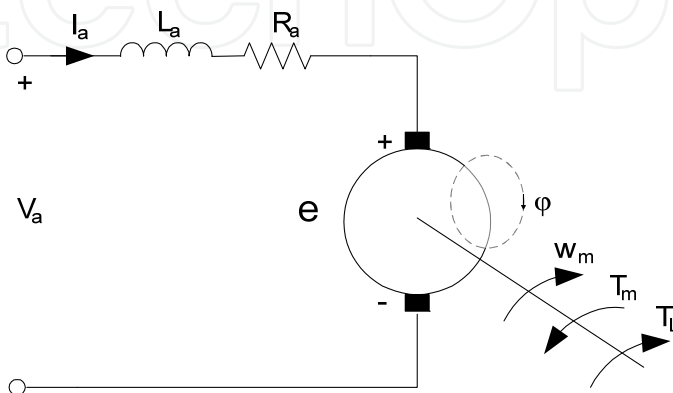
Fig. 8. Armature circuit model of dc machine
