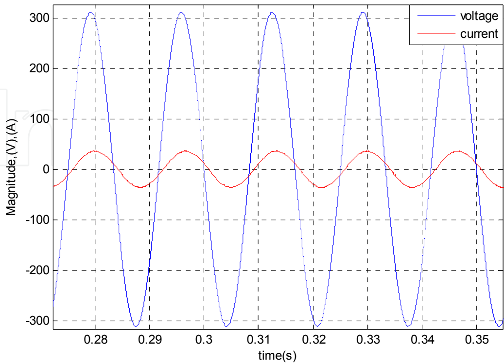
Fig. 16. One phase voltage and current
