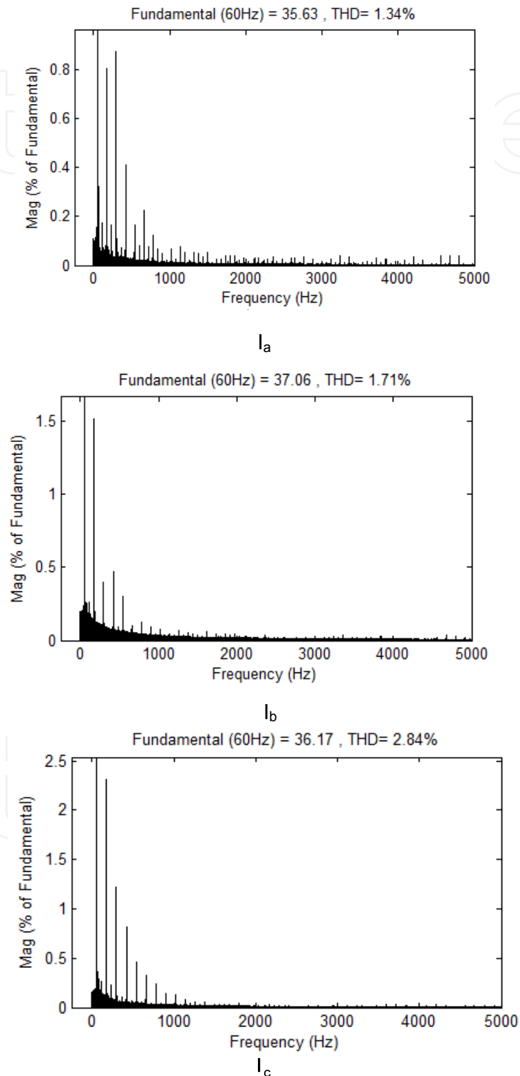
Fig. 18. Harmonic distortions of line currents
