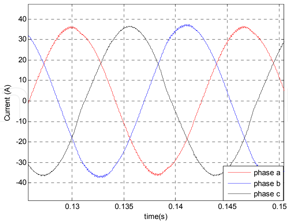
Fig. 17. Three-phase phase current
