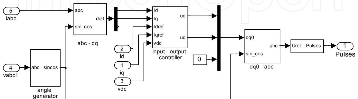
Fig. 11. Input-output controller diagram
