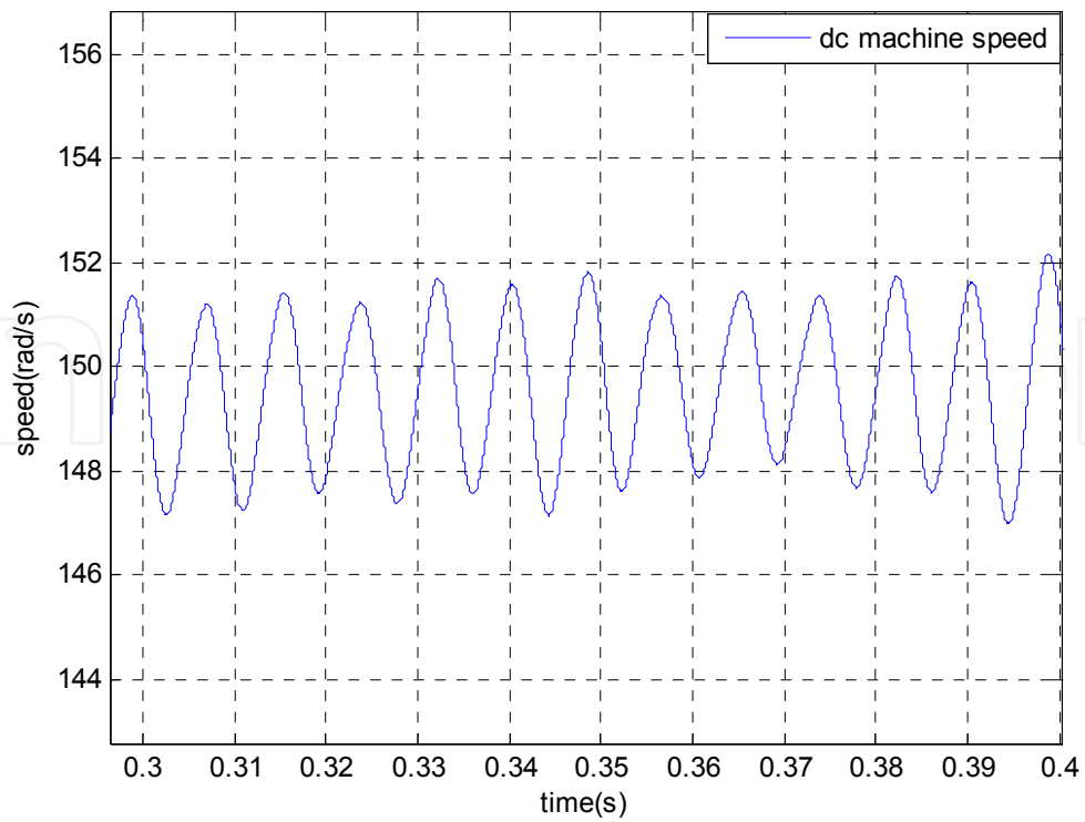
Fig. 15. Steady-state error of dc machine speed
