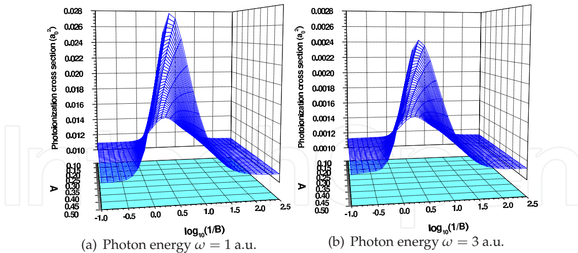
Fig. 6. Photoionization cross sections as functions of confining strengths ( A in atomic units) and quantum dot radii ( 1/B in atomic units) for finite oscillator potentials.
