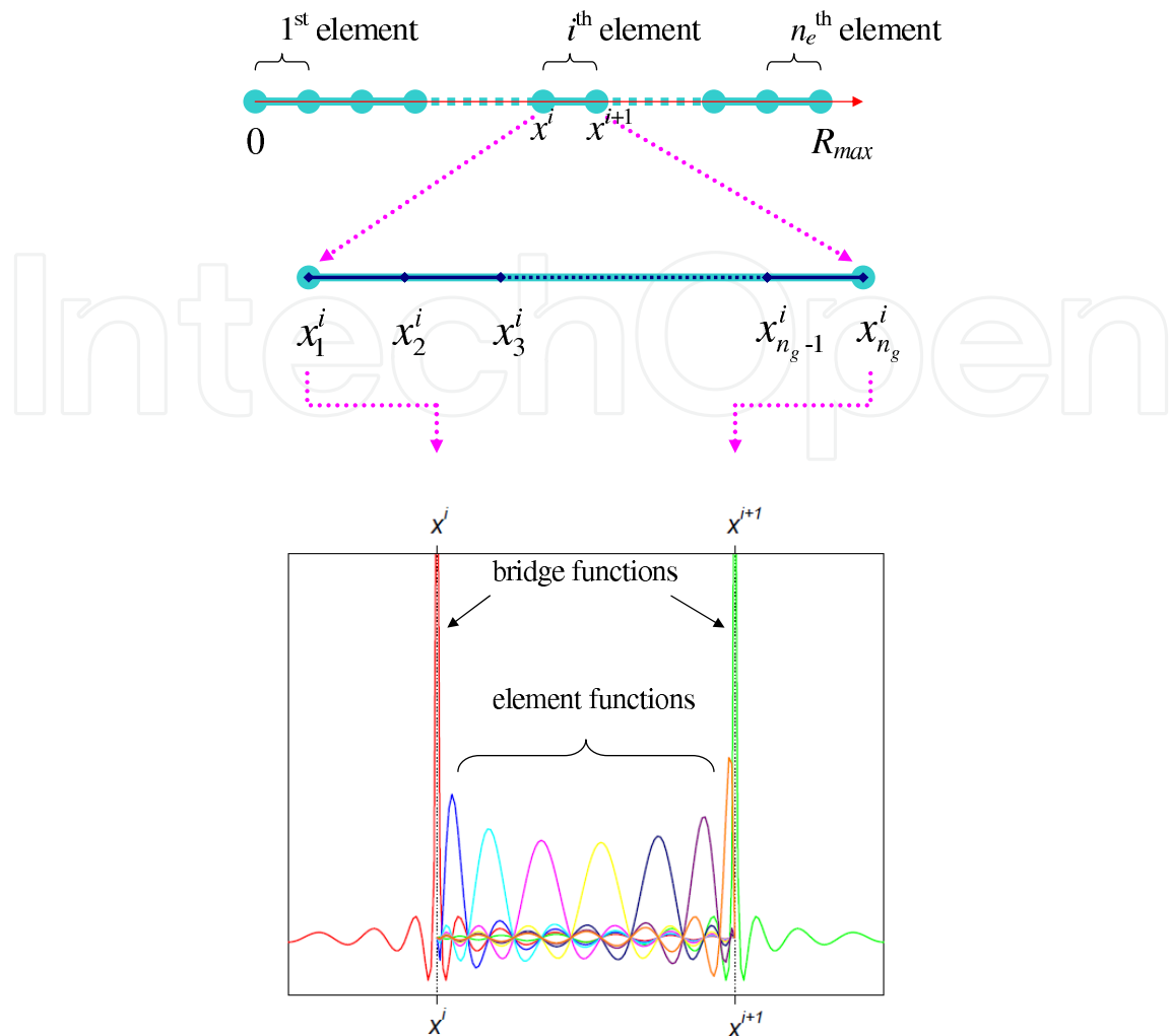
Fig. 2. Interval between 0 and R_{max} divided into n_e finite elements with n_g Gauss quadrature points and selected local basis functions (bridge and element functions) distributed in each finite element.
