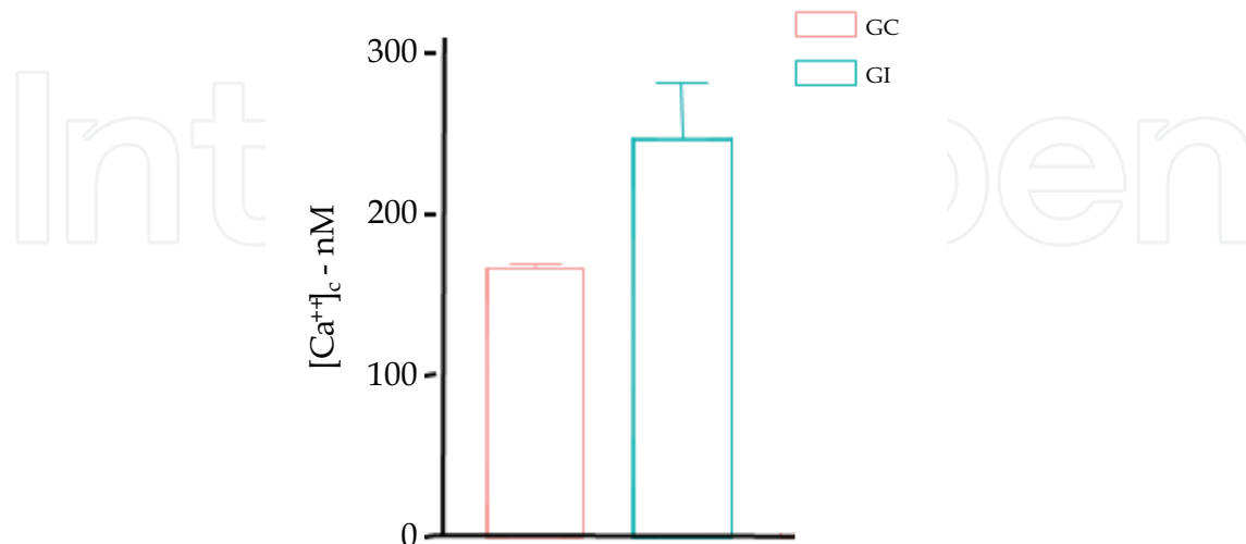
Fig. 8. Effect of \gamma radiation on basal intracellular \text{Ca}^{2+} concentration in mice granulocyte of the control (GC) and irradiated (GI) groups with doses of 700cCy - measured by fura-2 fluorophore. Statistical analysis: Newman Keuls. p < 0.05 , N = 4
