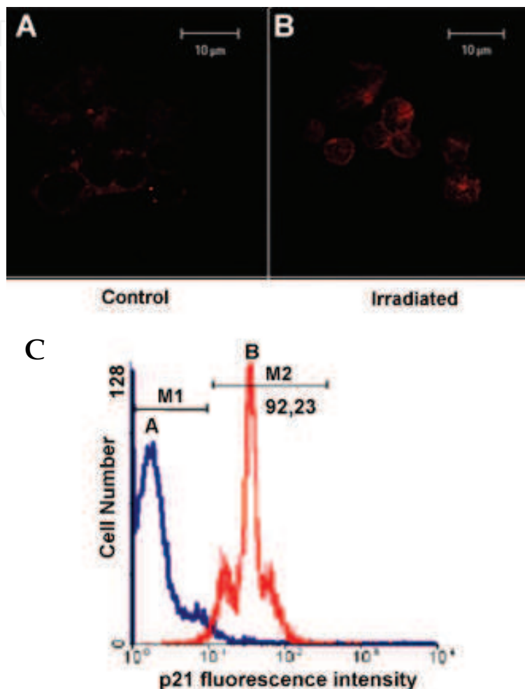
Fig. 4. (above – A and B) Confocal microscopy analysis: bone marrow cells of mice were immunostained in red-fluorescent. Specific staining using antibody p21 (red-fluorescent Alexa Fluor® 594). The irradiated group (B) shows an increase in fluorescence intensity and a change in p21 distribution when compared to the control group (A). (graph below-C) Flow cytometric analysis of p21 protein in paraformaldehyde-fixed cells harvested from mice femurs. Control group A (left) and irradiated group B (right). The bone marrow cells were analyzed 4h after radiation. The cells were pooled, washed, permeabilized with saponin, and stained with anti-p21 antibody and then analyzed by flow cytometry. Histograms were generated and analyzed using CellQuest cell cycle software. Percentage of cells showing fluorescence intensity. Histogram related to gated p21 positive bone marrow cells of GC and GI ( 89.8 \pm 5.3 ). Statistical analysis: Anova - Newman Keuls. p < 0.05 , N = 4 .
