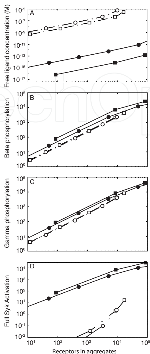
Fig. 11. Simulation of the effects of increasing the rate of serial engagement of bivalent and trivalent ligand by increasing the ligand-receptor dissociation constant, k_{\text{off}} . The four curves correspond to k_{+2}R_T = 1.0 \text{ s}^{-1} and bivalent (circles) and trivalent (squares) ligands with k_{\text{off}} = 0.01 \text{ s}^{-1} (solid lines and symbols) and 10 \text{ s}^{-1} (dashed lines and open symbols). The additional parameters used in the simulations are given in Table I of Faeder et al. (2003). The x-axis indicates levels of FcεRI aggregation, given as the number of receptors per cell in aggregates. One percent of the cell's receptors in aggregates corresponds to 4 \times 10^3 receptors. (A) Free ligand concentrations corresponding to specified levels of receptor aggregation. (B), (C), and (D) are respectively the predicted number of receptors per cell with the \beta ITAM phosphorylated, the \gamma ITAM phosphorylated, and Syk bound to the phosphorylated \gamma ITAM and transphosphorylated on its activation loop by another Syk.
