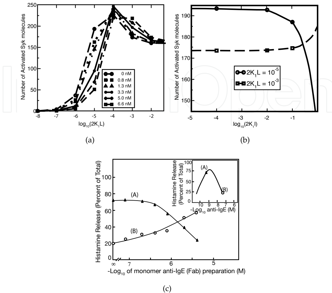
Fig. 4. (a) The effect of adding different concentrations of a monovalent IgE ligand on the extent of Syk activation at 2K_1L = 10^{-5} (Syk activation increases with 2K_1L ) and at 2K_1L = 10^{-3} (Syk activation decreases with 2K_1L ). The concentration of monovalent inhibitor (Fab fragments when the ligand is anti-IgE) present in the simulation is given in the figure. (b) The variation of the extent of Syk activation as a function of the concentration per cell of a monovalent inhibitor, I , at two ligand concentrations given by 2K_1L = 10^{-5} and 2K_1L = 10^{-3} . The ligand-receptor binding parameters used are k_{+1} = 2.5 \times 10^6 \text{ M}^{-1}\text{s}^{-1} , k_{+2} = 8 \times 10^{-9} \text{ cm}^2\text{s}^{-1} , k_{-1} = k_{-2} = 0.01\text{s}^{-1} . [\text{Syk}]_{\text{tot}} = 5 \times 10^3 per cell; [\text{Lyn}]_{\text{tot}} = 10^5 per cell; [\text{Fc}\epsilon\text{RI}]_{\text{tot}} = 10^5 per cell. (c) Modified Figure 1 from Magro and Alexander (Magro & Alexander, 1974). Plot of histamine release due to 5 \times 10^{-10} M anti-IgE (A) and 5 \times 10^{-8} M (B) incubated with increasing concentrations of monomer anti-IgE (Fab). The insert shows the positioning on the dose response curve of the two anti-IgE concentrations.
