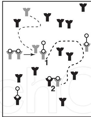
Fig. 16. At low ligand concentration, when most receptors are unbound, a receptor-ligand complex that dissociates from an aggregate (1), can rapidly enter a new aggregate (2), provided that the rate of cross-linking is greater than the rate of dissociation of its ligand-receptor bond. If this is not the case the ligand-receptor complex will be rapidly converted to a free receptor, reducing its chance of quickly finding a binding partner.
