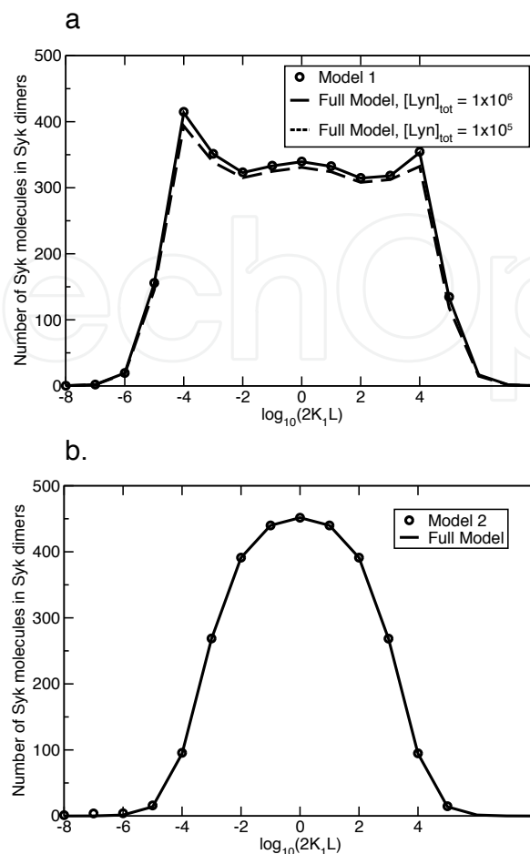
Fig. 6. Comparison of number of Syk dimers per cell obtained using reduced model 1 and 2, with the corresponding numbers obtained using the full model. [Syk]_{tot} = 7 \times 10^3 per cell; [FceRI]_{tot} = 10^5 per cell. We use the same ligand-receptor and Syk- p\gamma binding and unbinding parameters as in Table 2 for both the reduced models and the full model. (a) We consider two different total cellular concentrations of Lyn in the full model, [Lyn]_{tot} = 10^5 and [Lyn]_{tot} = 10^6 per cell. (b) Comparison of reduced model 2 to the full model when Lyn is in large excess and the rate of dephosphorylation is negligible ( [Lyn]_{tot} = 10^8 per cell, k_{-p} = 10^{-4} s^{-1} ).
