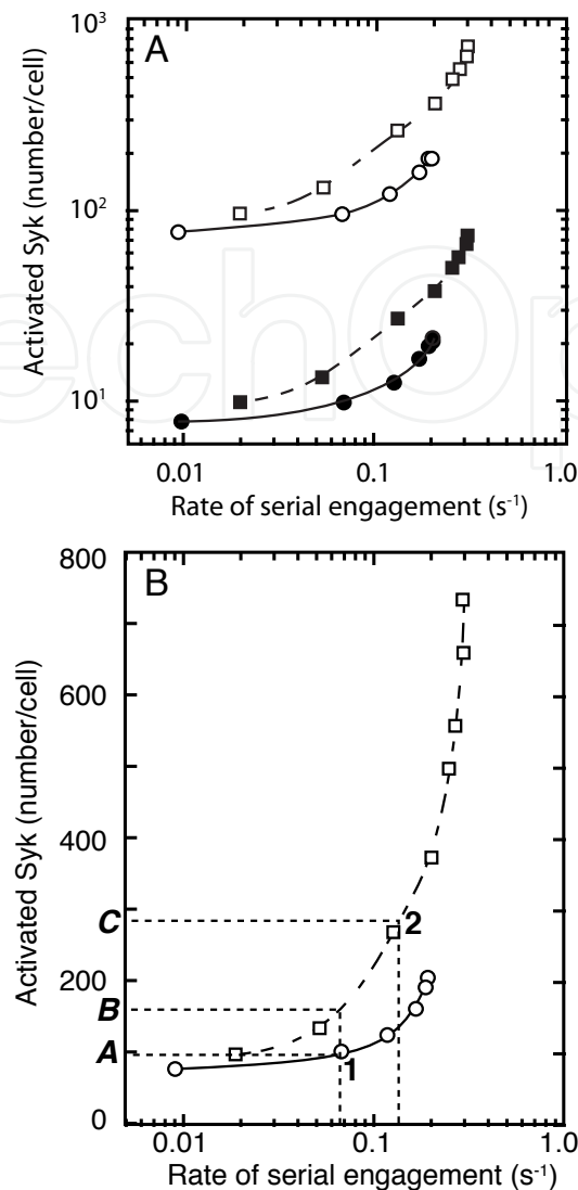
Fig. 13. Predicted number of activated Syk (Syk transphosphorylated by Syk) as a function of the rate of serial engagement. (A) The circles refer to bivalent ligand simulations and the squares to trivalent ligand simulations. Open and solid symbols refer to 1000 and 100 receptors in aggregates respectively. (B) Replot of the bivalent and trivalent curves in (A) for 1000 receptors in aggregates. The symbol 1 corresponds to a dimer with k_{+2R} = 0.01 \text{ s}^{-1} and k_{\text{off}} = 0.10 \text{ s}^{-1} . The symbol 2 corresponds to a trimer with the same rate constants. A = 100 , B = 161 and C = 290 activated Syk per cell. The net increase in activated Syk, (C - A) is 190 Syk per cell, of which C - B = 129 Syk per cell can be attributed to serial engagement.
