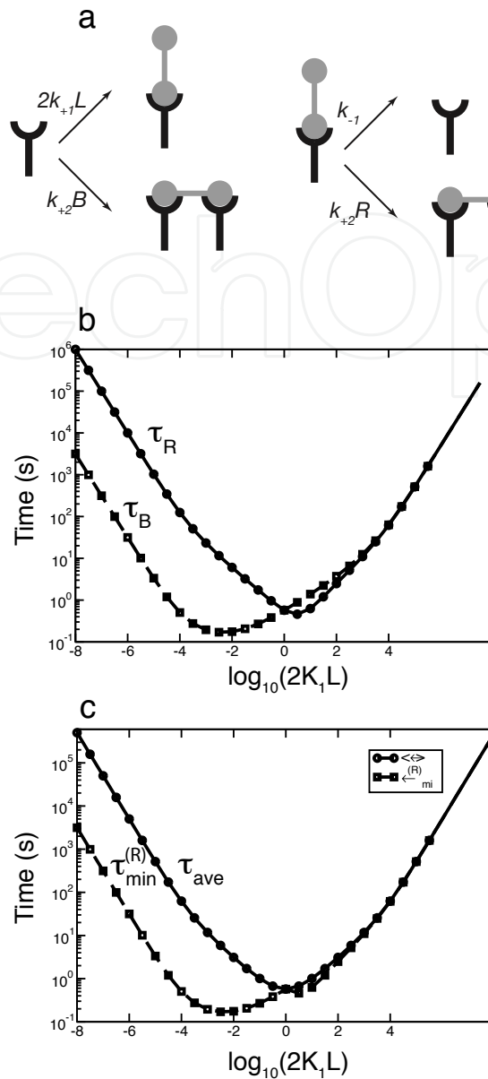
Fig. 9. (a) Rate constants that characterize the transitions that a free receptor and a bound receptor not in an aggregate can undergo. (b) The mean times for a free receptor ( \tau_R ) and a bound receptor ( \tau_B ) to find a partner and form a dimer as functions of the bivalent ligand concentration. (c) The mean \tau_{ave} of \tau_R and \tau_B and the minimum \tau_{min}^{(R)} of \tau_R and \tau_B as a function of the ligand concentration. In parts (b) and (c), the ligand receptor binding and cross-linking parameters are taken from Table 2 and [Fc\epsilon RI]_{tot} = 10^5 per cell.
