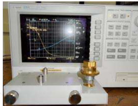
Fig. 9. Impedance meter Agilent 4294A and magnetic module
