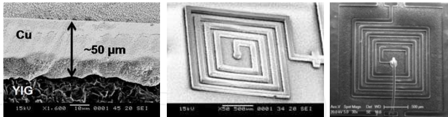
Fig. 19. SEM images of the micro-fabricated inductor
