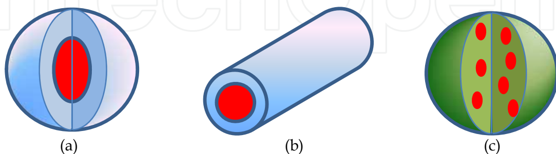
Fig. 1. Three types of the magnetolectric nanoparticles: spherical core-shell nanoparticles with magnetostrictive core encapsulated in piezoelectric shell (a), cylindrical core-shell nanoparticle with magnetostrictive rod and piezoelectric coating (b) and a composite superparticle with magnetic nanoparticles embedded into piezo-polymer or piezo-ceramics (c).
