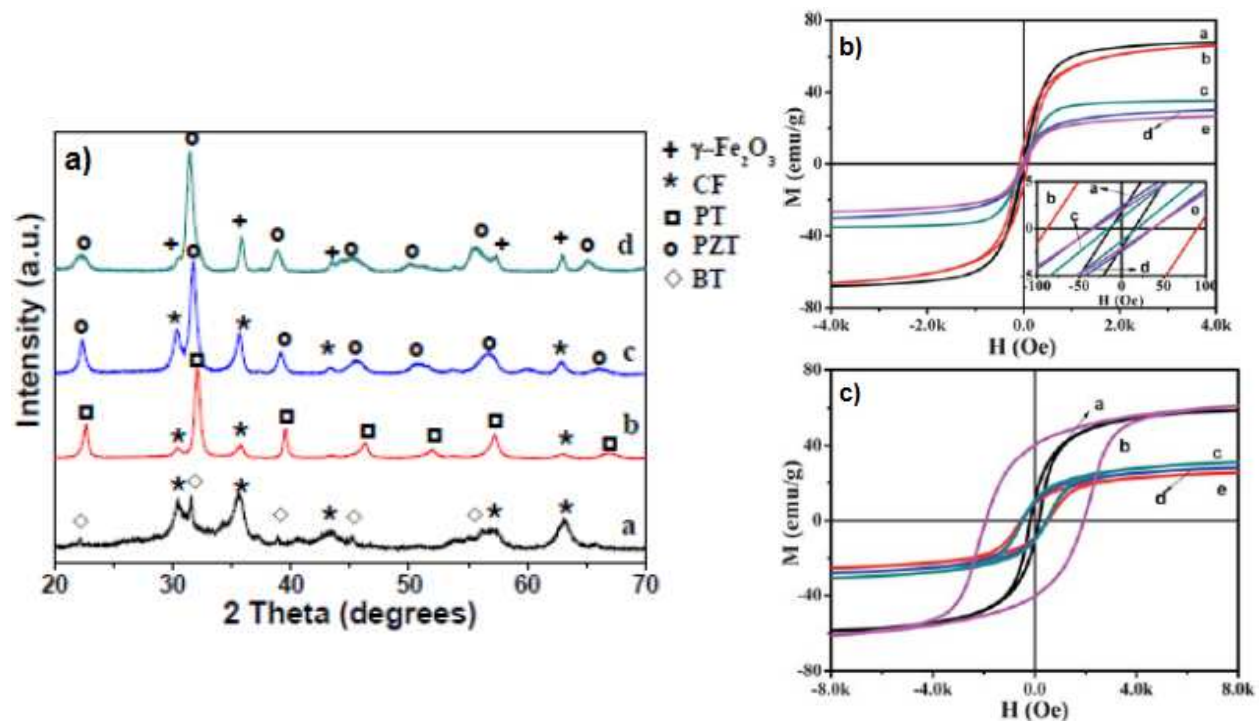
Fig. 8. XRD patterns of core-shell nanostructured powders of SEM images of CoFe 2 O 4 /BaTiO 3 (a); CoFe 2 O 4 /PbTiO 3 ; Fe 3 O 4 (b); CoFe 2 O 4 /Pb(Ti, Zr)TiO 3 (c) and γ-Fe 2 O 3 /PbTiO 3 (d) nanoparticles. Magnetic hysteresis loops of Fe 3 O 4 (a); γ-Fe 2 O 3 (b); Fe 3 O 4 /PbTiO 3 (c); γ-Fe 2 O 3 /PbTiO 3 (e); γ-Fe 2 O 3 /Pb(Ti, Zr)O 3 nanoparticles (upper panel) and the as-prepared CoFe 2 O 4 nanoparticles (a) and after annealing at 600 °C (b) and CoFe 2 O 4 /BaTiO 3 (c); CoFe 2 O 4 /PbTiO 3 (d) and CoFe 2 O 4 /Pb(Ti, Zr)O 3 (e) nanopowders, respectively
