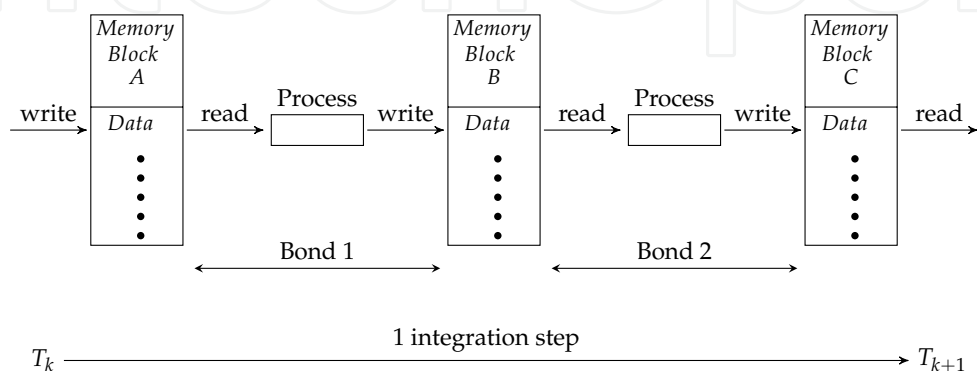
Fig. 10. Propagation of data in an integral time step
