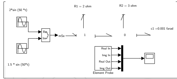
(b) Bond graph model of RC circuit
