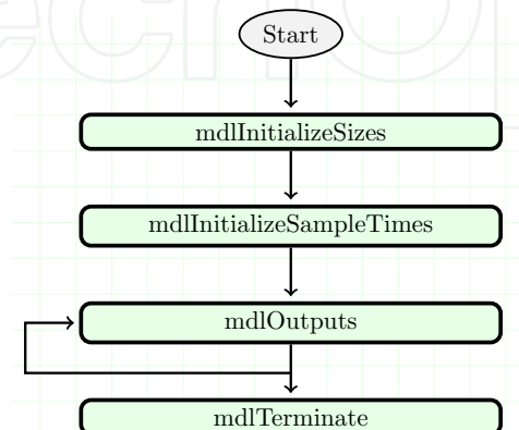
Fig. 6. C MEX S-function timestwo Blocks
