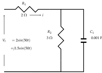
(a) RC circuit
