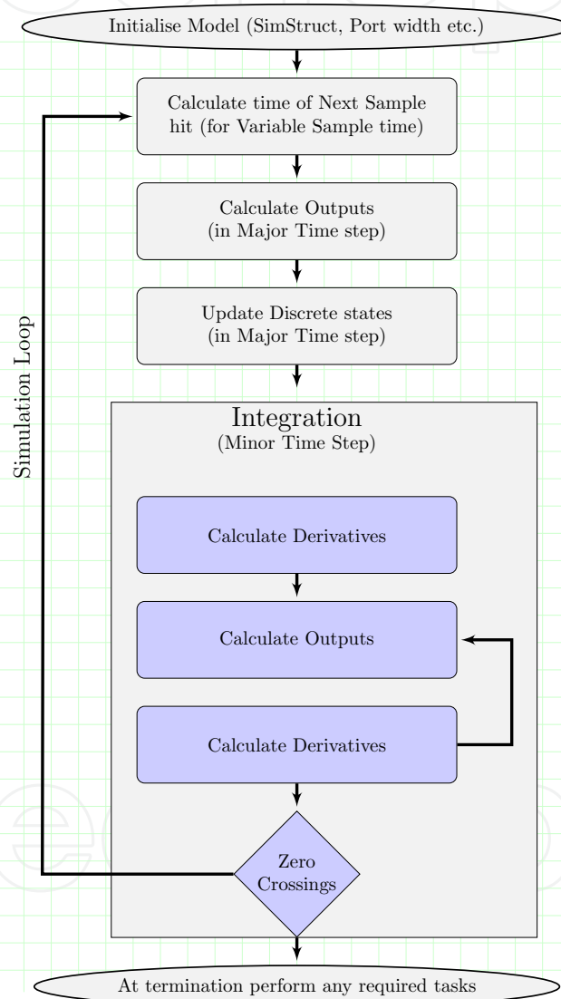
Fig. 2. S-function simulation cycle
