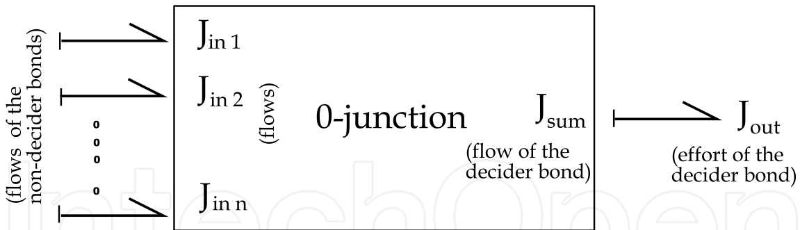
Fig. 8. 0-junction
