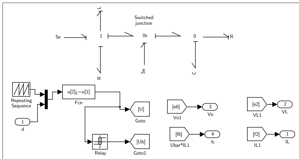
(e) Boost converter model built using switched junction
