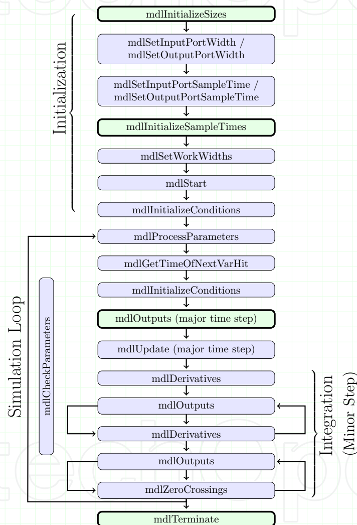
Fig. 3. Calling sequence of C MEX S-function Blocks
