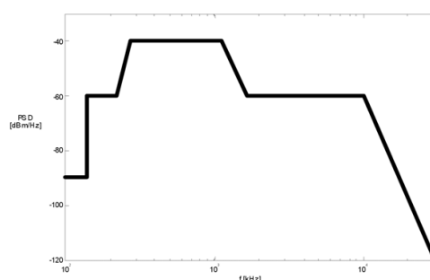
Fig. 3. The PSD mask of the VDSL signal for the FTTEEx variation with narrowband services and the ADSL presence
