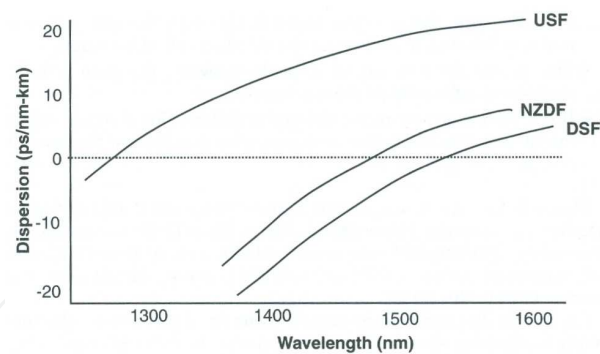
Fig. 15. Wavelength characteristics of the dispersion for USF, NZDF and DSF fibers
