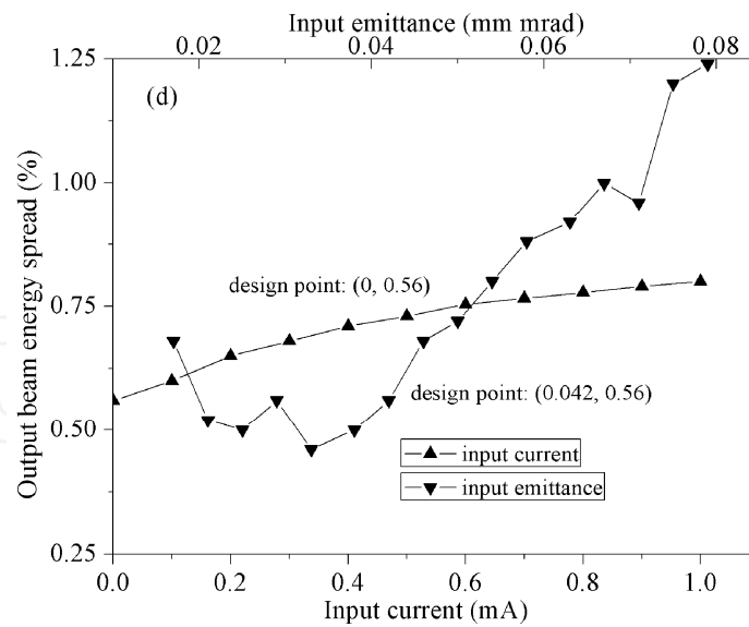
Fig. 3. Stability studies of the beam dynamics design of the ladder IH-RFQ: beam transmission efficiency versus Twiss parameters in (a), output beam energy spread versus Twiss parameters in (b), beam transmission efficiency versus input current and emittance in (c), output beam energy spread versus input current and emittance in (d).
