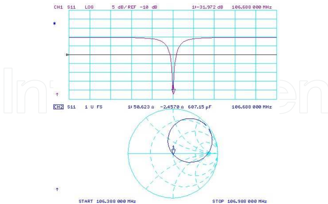
Fig. 12. The critical coupling point of the ladder IH-RFQ: the S_{11} parameter (up) and Smith Chart (down).
