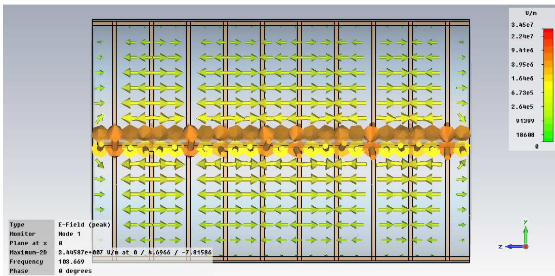
(a) Electric field among electrodes (up) and stems (bottom) of the ladder IH-RFQ
