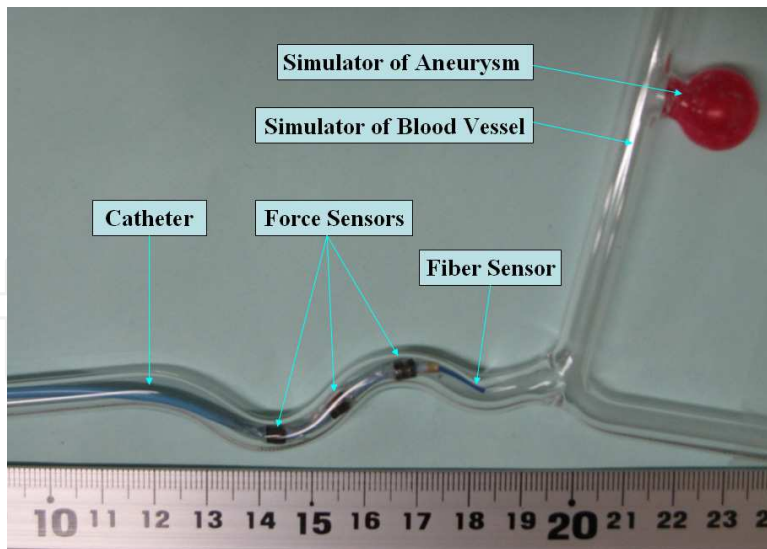
Fig. 15. Experimental set up
