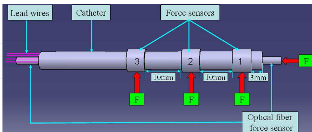
Fig. 5. Prototype of developed force sensors system
